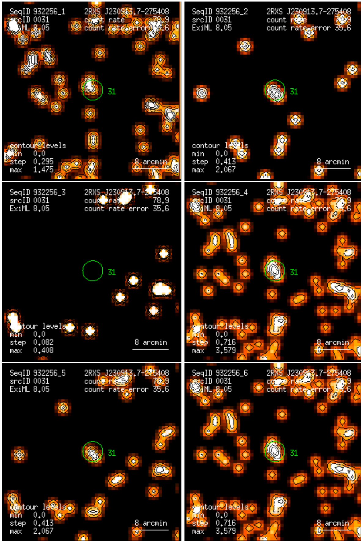
Figure 31: RASS 932256: detection 0031: band rate images, Gaussian filter: (1) PSPC channels 11 – 41, (2) 52 – 90, (3) 91 – 201, (4) 11 – 235, (5) 52 – 201, (6) 11 – 201. Broad band rates in counts/ks. Band rate contour levels in counts/ks/arcmin 2 .
