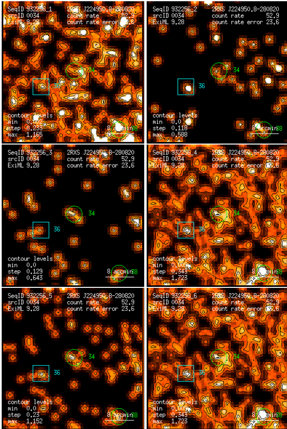
Figure 34: RASS 932256: detection 0034: band rate images, Gaussian filter: (1) PSPC channels 11 – 41, (2) 52 – 90, (3) 91 – 201, (4) 11 – 235, (5) 52 – 201, (6) 11 – 201. Broad band rates in counts/ks. Band rate contour levels in counts/ks/arcmin 2 .
