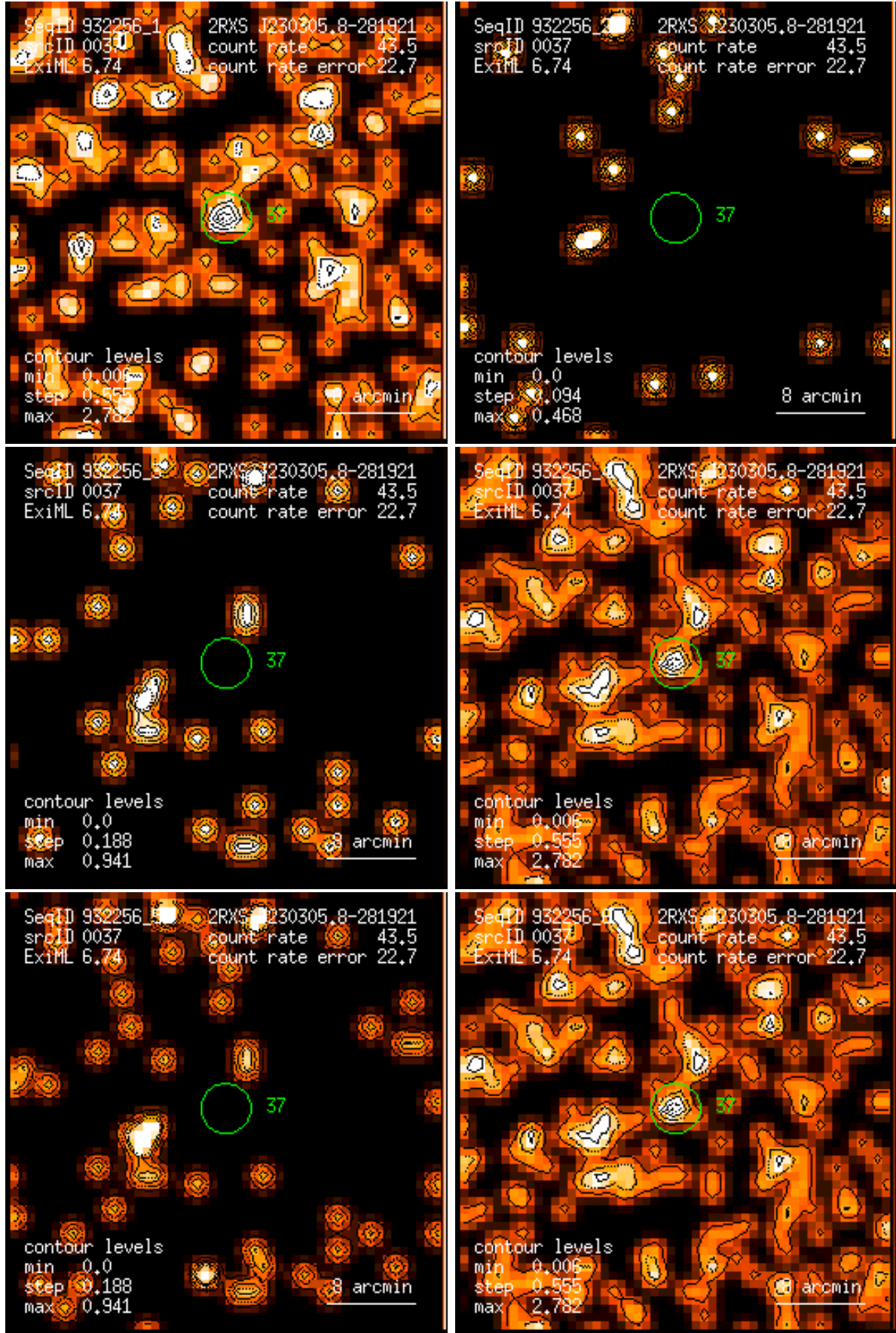
Figure 37: RASS 932256: detection 0037: band rate images, Gaussian filter: (1) PSPC channels 11 – 41, (2) 52 – 90, (3) 91 – 201, (4) 11 – 235, (5) 52 – 201, (6) 11 – 201. Broad band rates in counts/ks. Band rate contour levels in counts/ks/arcmin 2 .
