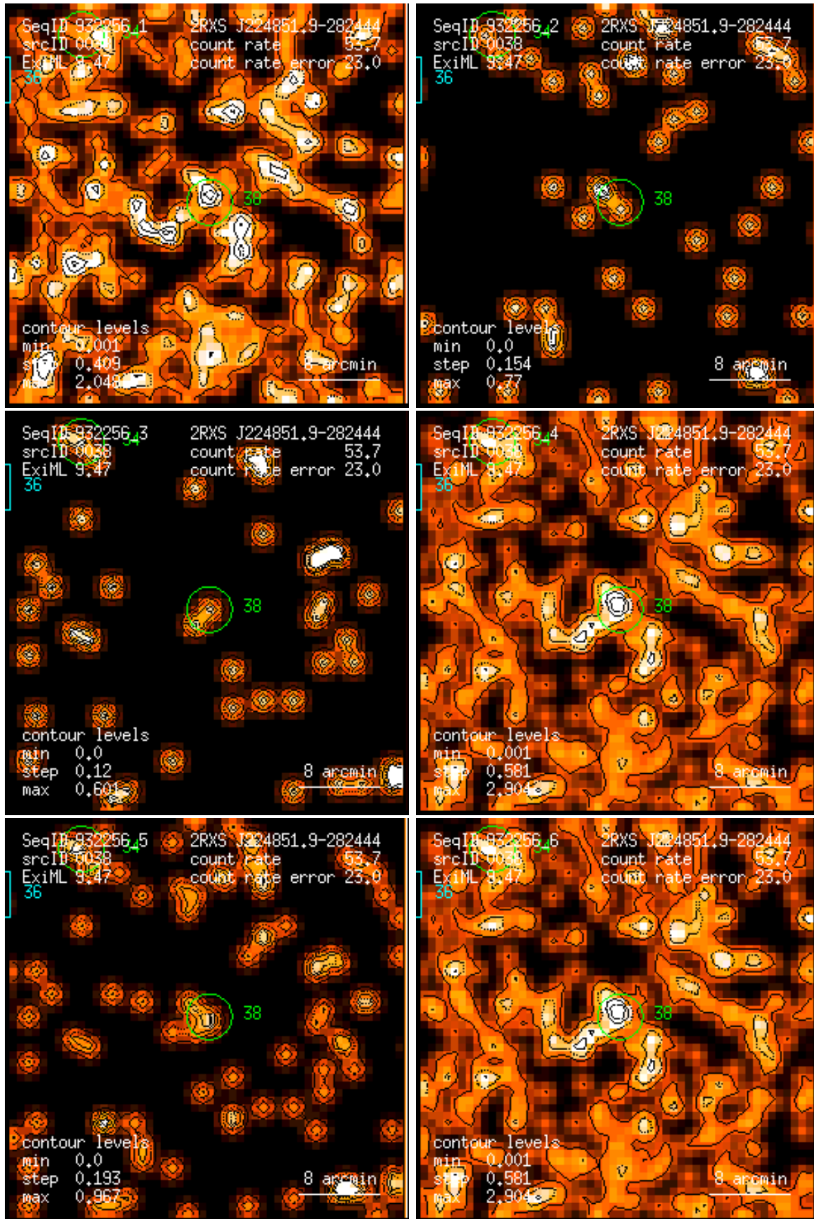
Figure 38: RASS 932256: detection 0038: band rate images, Gaussian filter: (1) PSPC channels 11 – 41, (2) 52 – 90, (3) 91 – 201, (4) 11 – 235, (5) 52 – 201, (6) 11 – 201. Broad band rates in counts/ks. Band rate contour levels in counts/ks/arcmin 2 .
