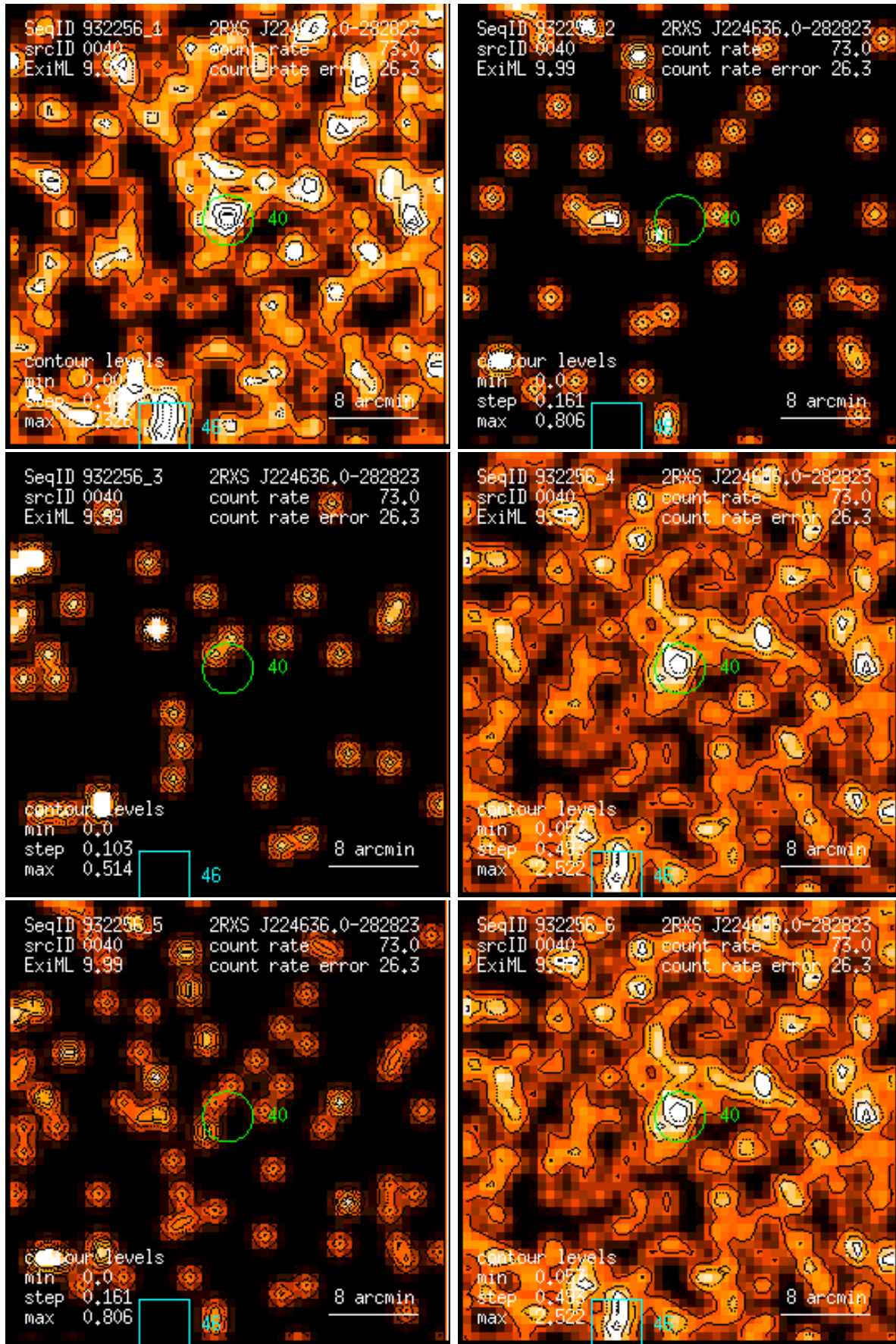
Figure 40: RASS 932256: detection 0040: band rate images, Gaussian filter: (1) PSPC channels 11 – 41, (2) 52 – 90, (3) 91 – 201, (4) 11 – 235, (5) 52 – 201, (6) 11 – 201. Broad band rates in counts/ks. Band rate contour levels in counts/ks/arcmin 2 .
