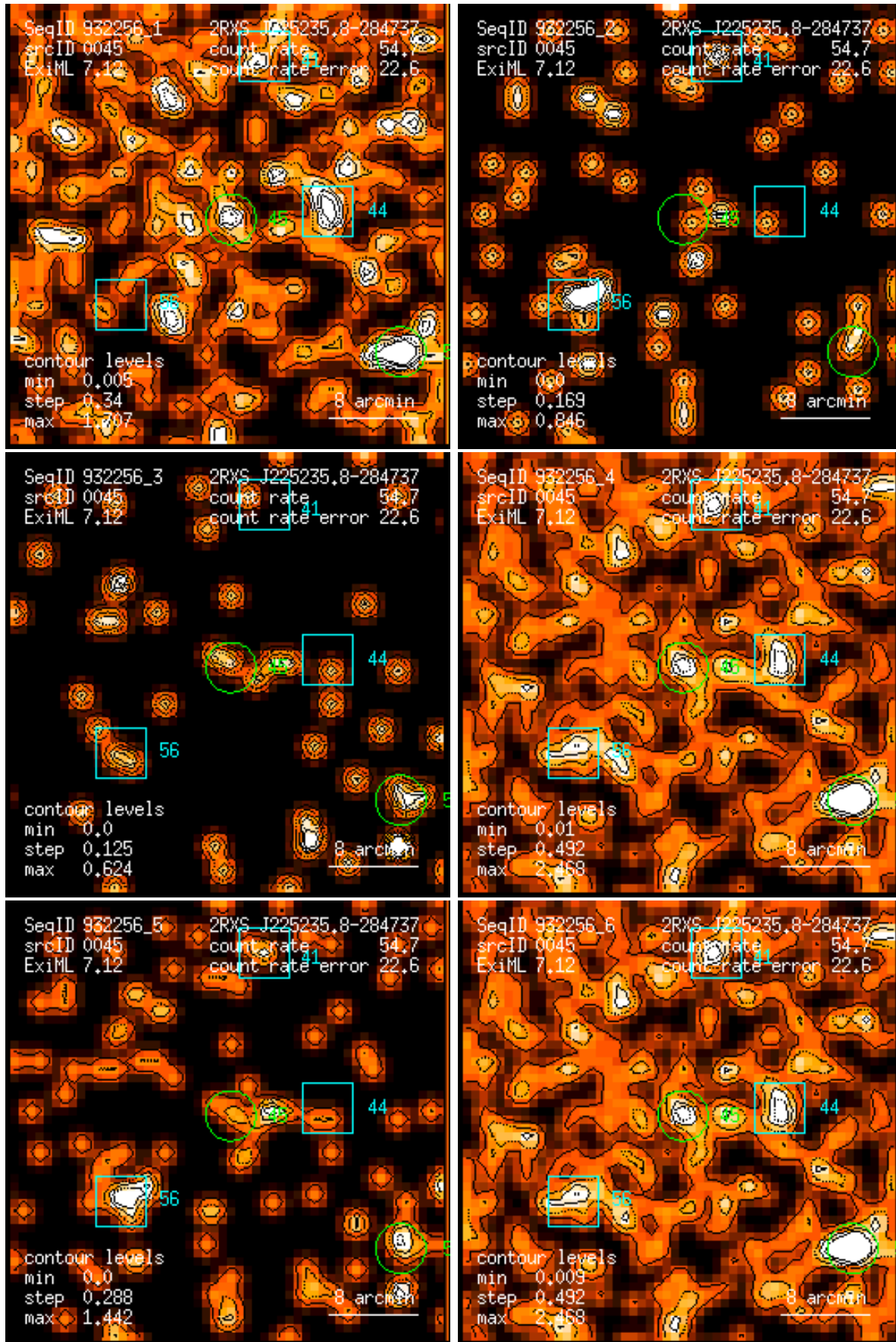
Figure 45: RASS 932256: detection 0045: band rate images, Gaussian filter: (1) PSPC channels 11 – 41, (2) 52 – 90, (3) 91 – 201, (4) 11 – 235, (5) 52 – 201, (6) 11 – 201. Broad band rates in counts/ks. Band rate contour levels in counts/ks/arcmin 2 .
