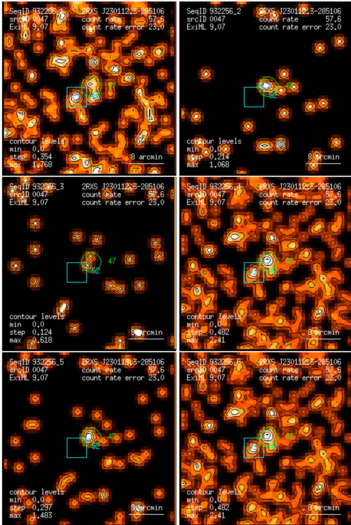
Figure 47: RASS 932256: detection 0047: band rate images, Gaussian filter: (1) PSPC channels 11 – 41, (2) 52 – 90, (3) 91 – 201, (4) 11 – 235, (5) 52 – 201, (6) 11 – 201. Broad band rates in counts/ks. Band rate contour levels in counts/ks/arcmin 2 .
