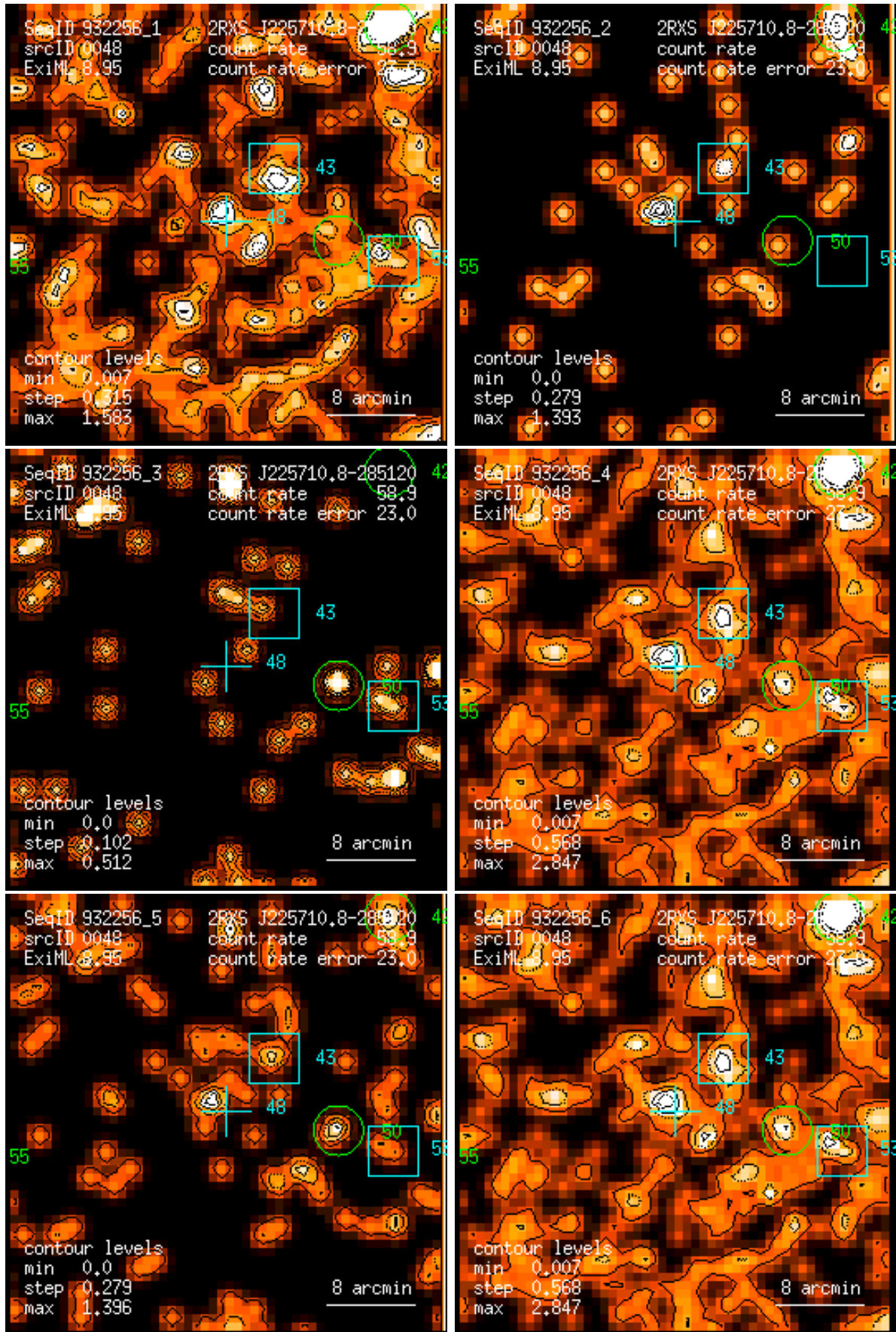
Figure 48: RASS 932256: detection 0048: band rate images, Gaussian filter: (1) PSPC channels 11 – 41, (2) 52 – 90, (3) 91 – 201, (4) 11 – 235, (5) 52 – 201, (6) 11 – 201. Broad band rates in counts/ks. Band rate contour levels in counts/ks/arcmin 2 .
