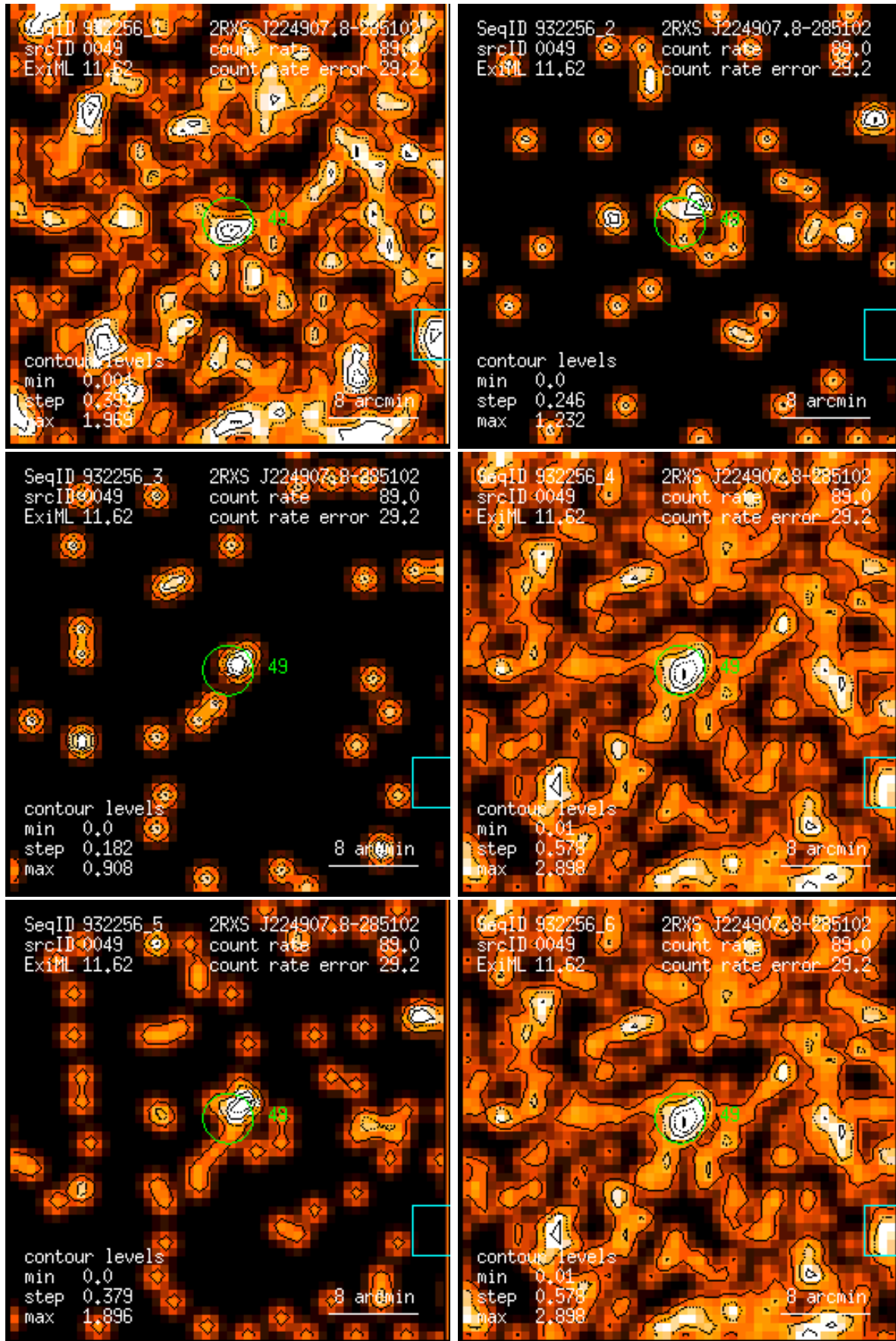
Figure 49: RASS 932256: detection 0049: band rate images, Gaussian filter: (1) PSPC channels 11 – 41, (2) 52 – 90, (3) 91 – 201, (4) 11 – 235, (5) 52 – 201, (6) 11 – 201. Broad band rates in counts/ks. Band rate contour levels in counts/ks/arcmin 2 .
