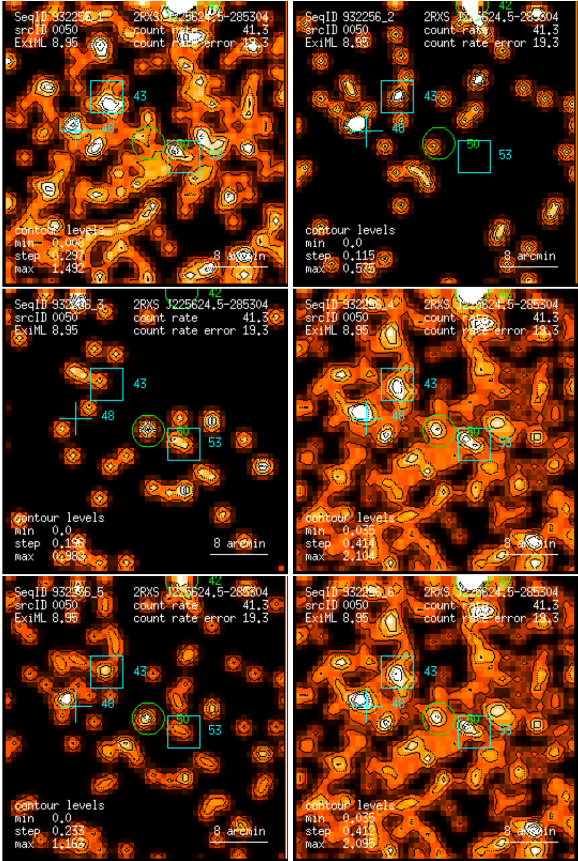
Figure 50: RASS 932256: detection 0050: band rate images, Gaussian filter: (1) PSPC channels 11 – 41, (2) 52 – 90, (3) 91 – 201, (4) 11 – 235, (5) 52 – 201, (6) 11 – 201. Broad band rates in counts/ks. Band rate contour levels in counts/ks/arcmin 2 .
