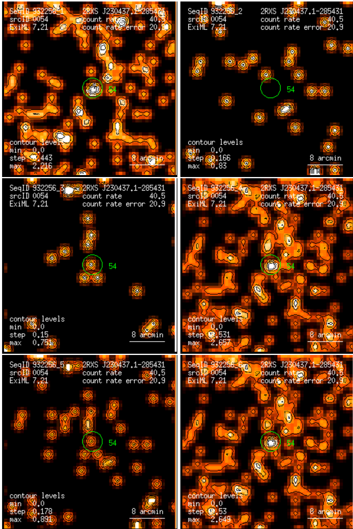
Figure 54: RASS 932256: detection 0054: band rate images, Gaussian filter: (1) PSPC channels 11 – 41, (2) 52 – 90, (3) 91 – 201, (4) 11 – 235, (5) 52 – 201, (6) 11 – 201. Broad band rates in counts/ks. Band rate contour levels in counts/ks/arcmin 2 .
