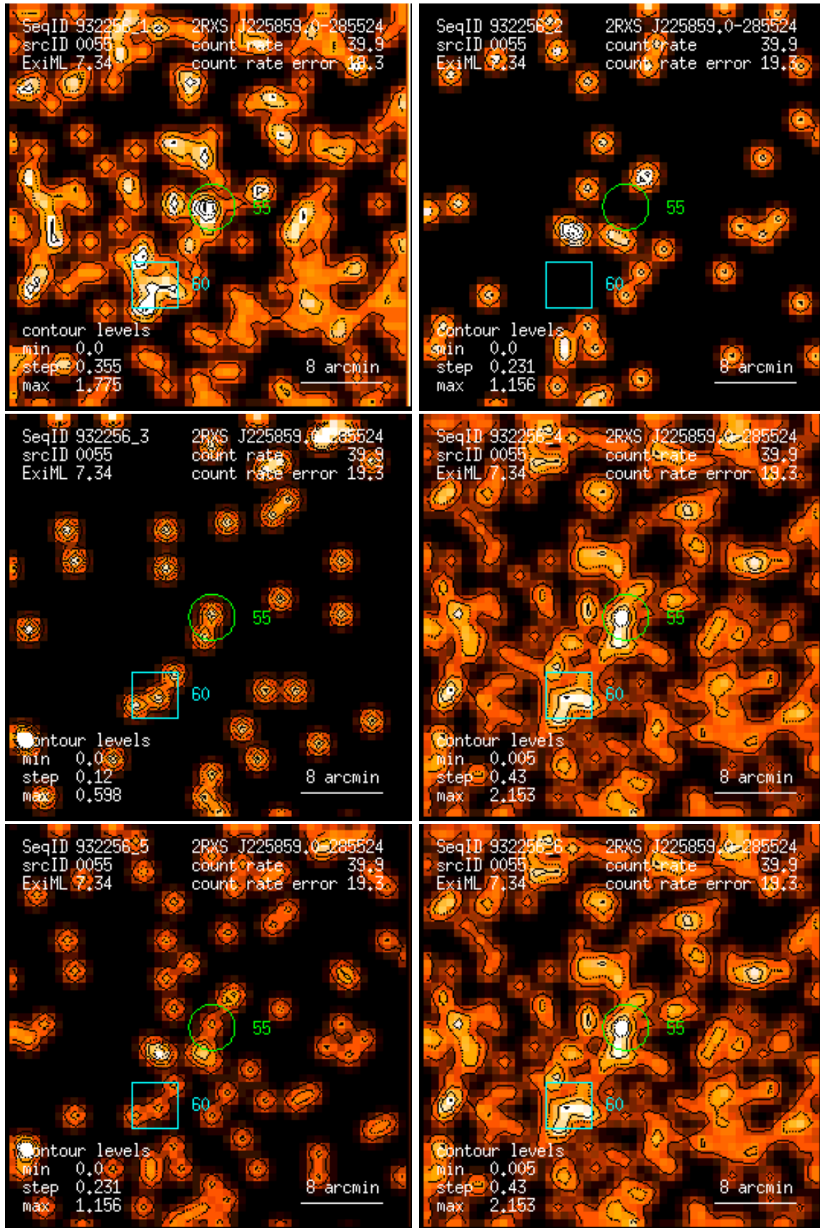
Figure 55: RASS 932256: detection 0055: band rate images, Gaussian filter: (1) PSPC channels 11 – 41, (2) 52 – 90, (3) 91 – 201, (4) 11 – 235, (5) 52 – 201, (6) 11 – 201. Broad band rates in counts/ks. Band rate contour levels in counts/ks/arcmin 2 .
