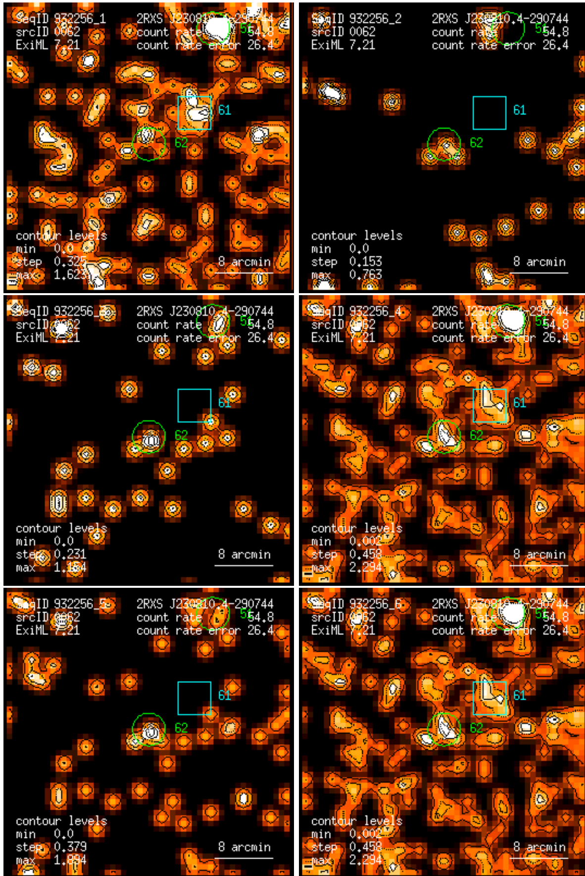
Figure 62: RASS 932256: detection 0062: band rate images, Gaussian filter: (1) PSPC channels 11 – 41, (2) 52 – 90, (3) 91 – 201, (4) 11 – 235, (5) 52 – 201, (6) 11 – 201. Broad band rates in counts/ks. Band rate contour levels in counts/ks/arcmin 2 .
