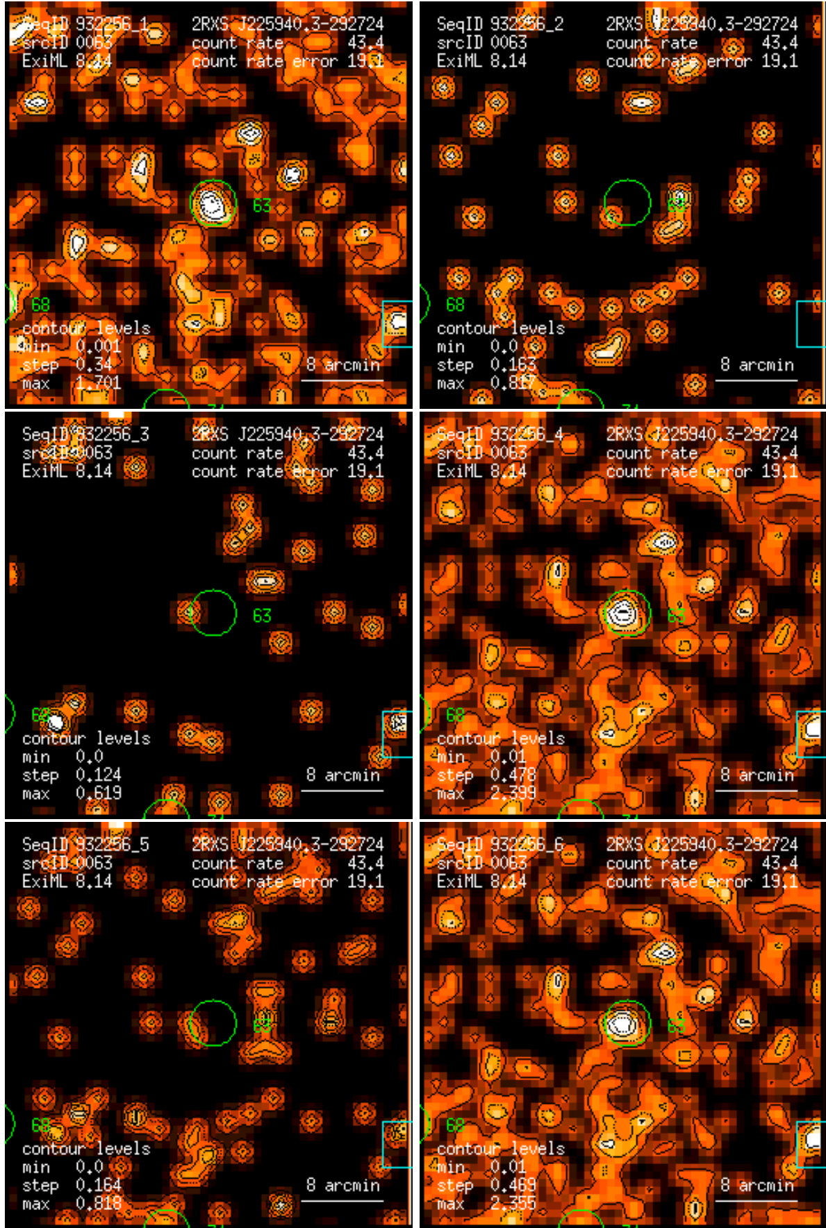
Figure 63: RASS 932256: detection 0063: band rate images, Gaussian filter: (1) PSPC channels 11 – 41, (2) 52 – 90, (3) 91 – 201, (4) 11 – 235, (5) 52 – 201, (6) 11 – 201. Broad band rates in counts/ks. Band rate contour levels in counts/ks/arcmin 2 .
