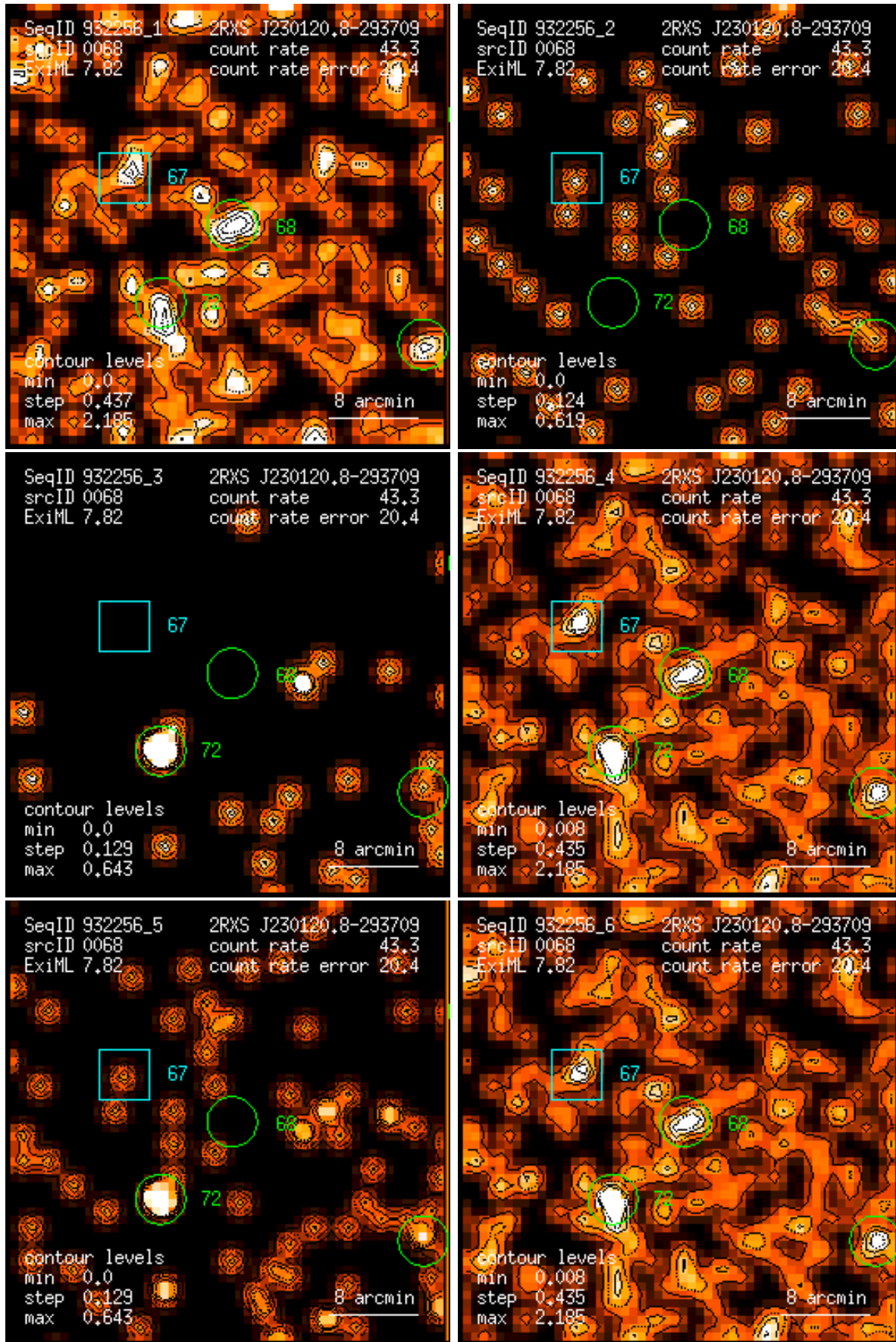
Figure 68: RASS 932256: detection 0068: band rate images, Gaussian filter: (1) PSPC channels 11 – 41, (2) 52 – 90, (3) 91 – 201, (4) 11 – 235, (5) 52 – 201, (6) 11 – 201. Broad band rates in counts/ks. Band rate contour levels in counts/ks/arcmin 2 .
