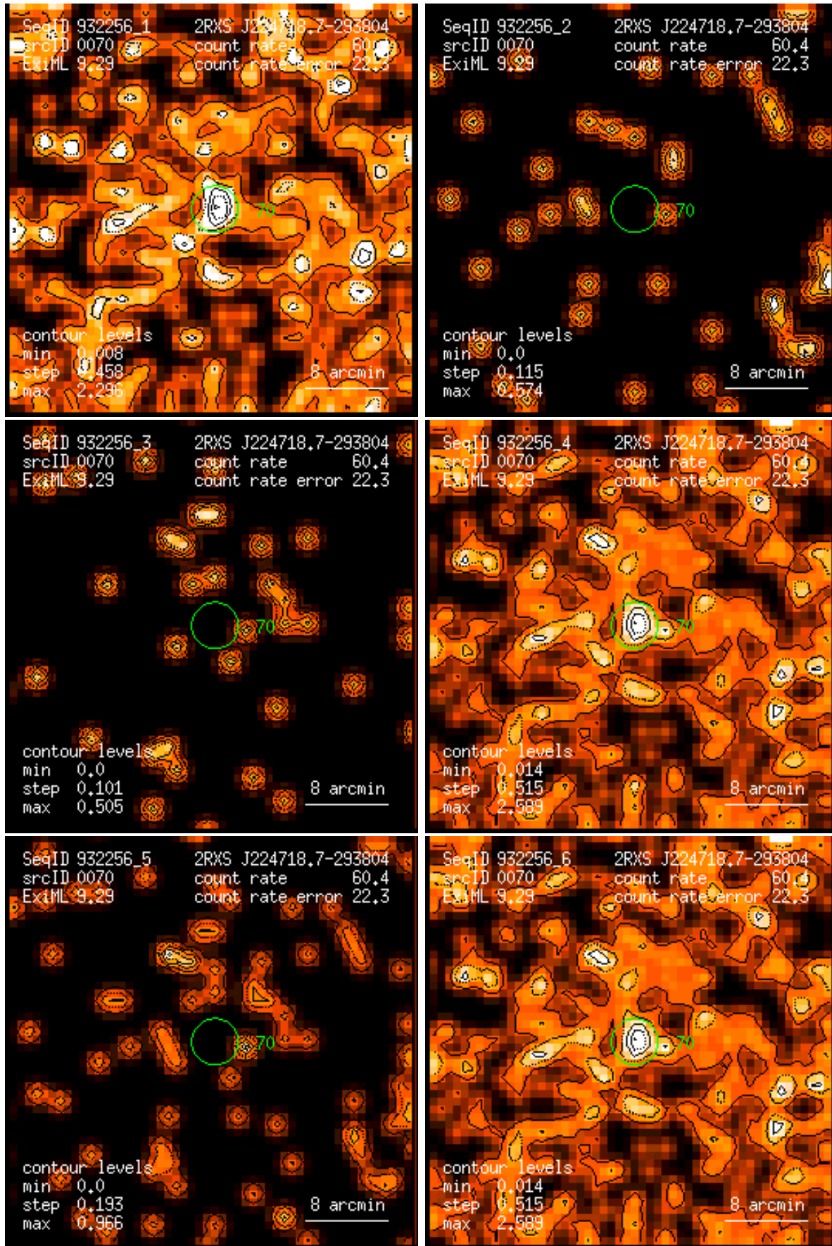
Figure 70: RASS 932256: detection 0070: band rate images, Gaussian filter: (1) PSPC channels 11 – 41, (2) 52 – 90, (3) 91 – 201, (4) 11 – 235, (5) 52 – 201, (6) 11 – 201. Broad band rates in counts/ks. Band rate contour levels in counts/ks/arcmin 2 .
