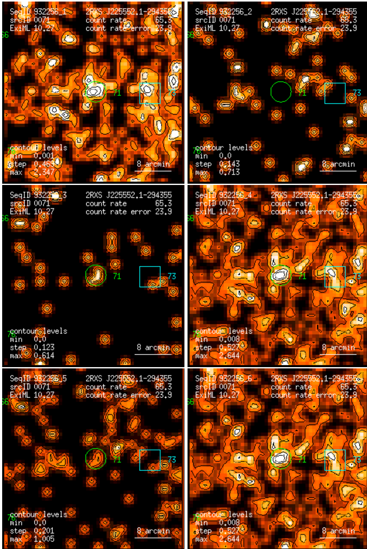
Figure 71: RASS 932256: detection 0071: band rate images, Gaussian filter: (1) PSPC channels 11 – 41, (2) 52 – 90, (3) 91 – 201, (4) 11 – 235, (5) 52 – 201, (6) 11 – 201. Broad band rates in counts/ks. Band rate contour levels in counts/ks/arcmin 2 .
