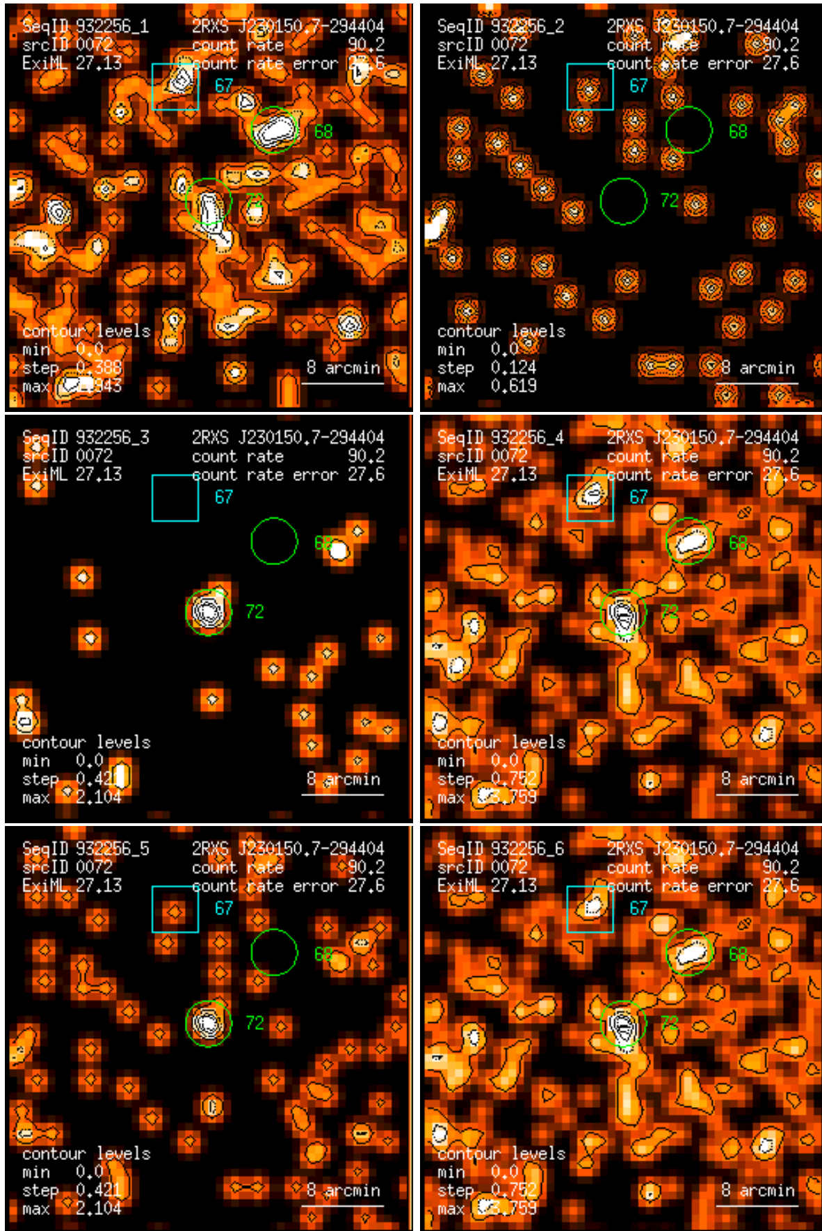
Figure 72: RASS 932256: detection 0072: band rate images, Gaussian filter: (1) PSPC channels 11 – 41, (2) 52 – 90, (3) 91 – 201, (4) 11 – 235, (5) 52 – 201, (6) 11 – 201. Broad band rates in counts/ks. Band rate contour levels in counts/ks/arcmin 2 .
