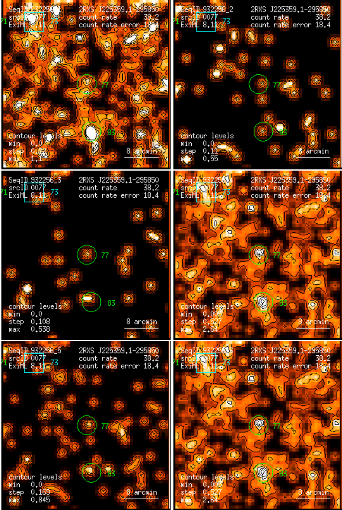
Figure 77: RASS 932256: detection 0077: band rate images, Gaussian filter: (1) PSPC channels 11 – 41, (2) 52 – 90, (3) 91 – 201, (4) 11 – 235, (5) 52 – 201, (6) 11 – 201. Broad band rates in counts/ks. Band rate contour levels in counts/ks/arcmin 2 .
