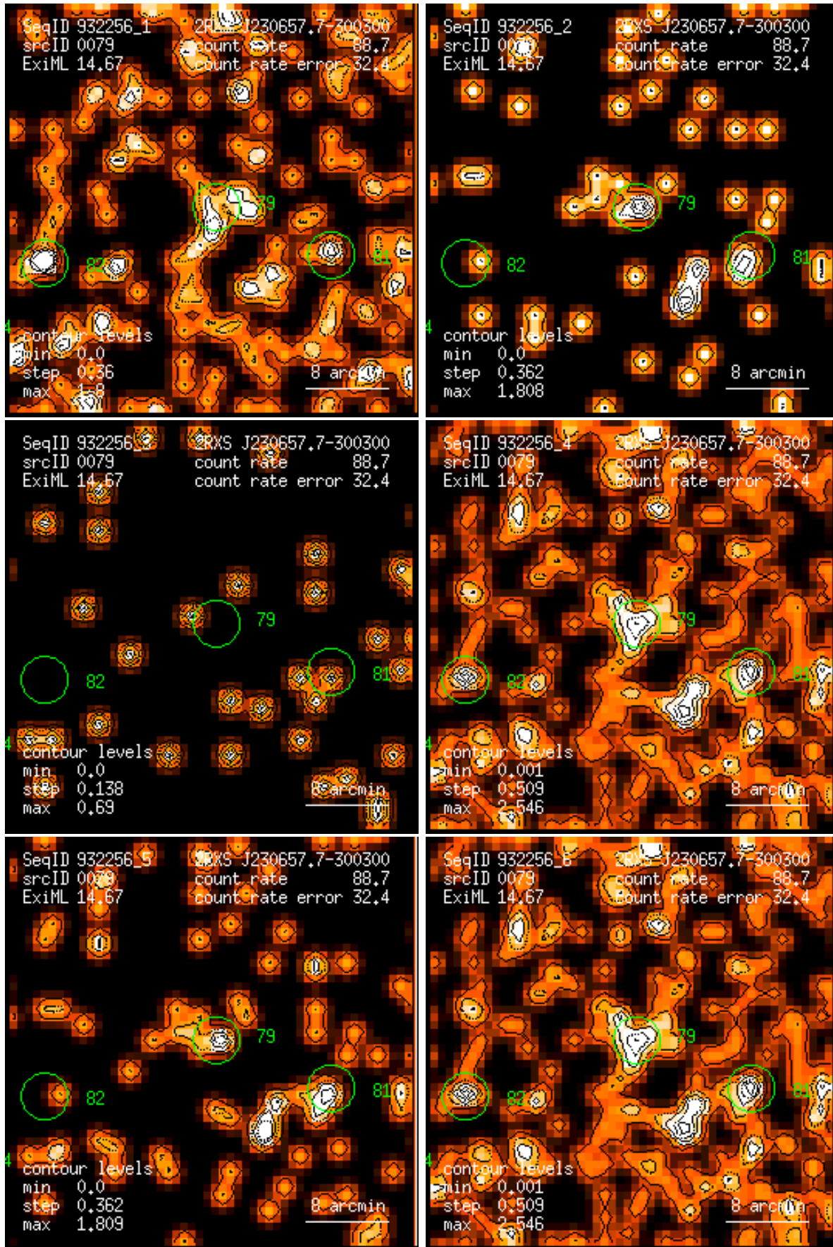
Figure 79: RASS 932256: detection 0079: band rate images, Gaussian filter: (1) PSPC channels 11 – 41, (2) 52 – 90, (3) 91 – 201, (4) 11 – 235, (5) 52 – 201, (6) 11 – 201. Broad band rates in counts/ks. Band rate contour levels in counts/ks/arcmin 2 .
