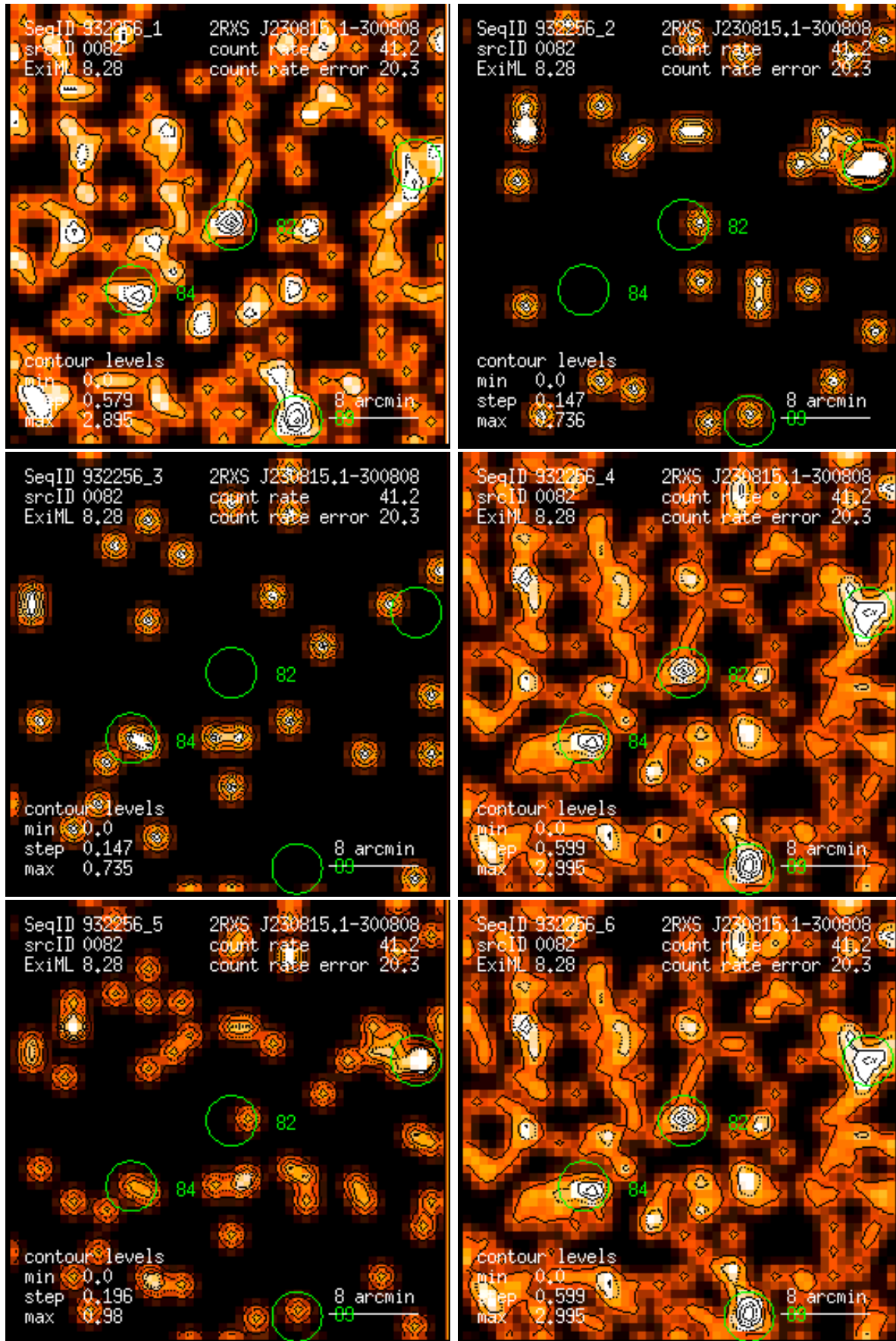
Figure 82: RASS 932256: detection 0082: band rate images, Gaussian filter: (1) PSPC channels 11 – 41, (2) 52 – 90, (3) 91 – 201, (4) 11 – 235, (5) 52 – 201, (6) 11 – 201. Broad band rates in counts/ks. Band rate contour levels in counts/ks/arcmin 2 .
