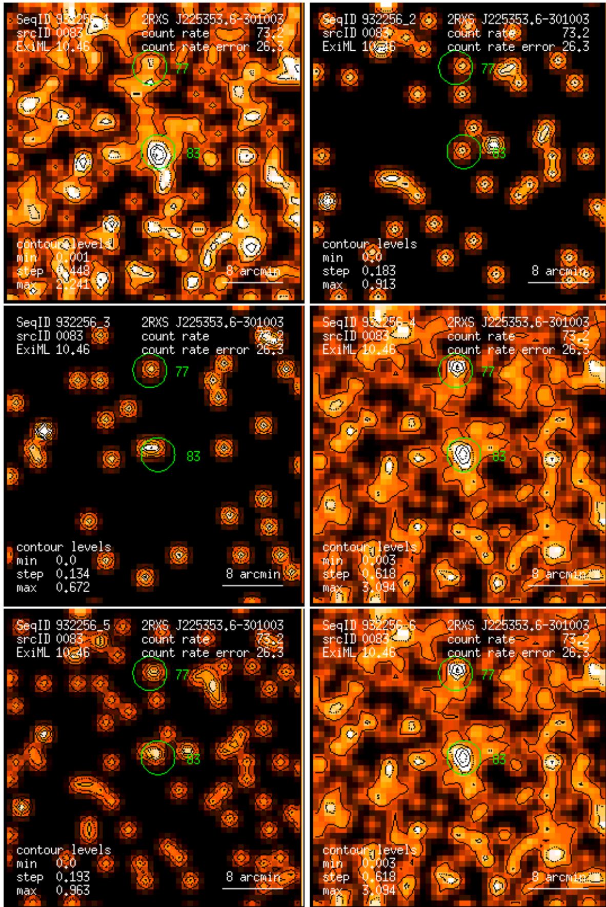
Figure 83: RASS 932256: detection 0083: band rate images, Gaussian filter: (1) PSPC channels 11 – 41, (2) 52 – 90, (3) 91 – 201, (4) 11 – 235, (5) 52 – 201, (6) 11 – 201. Broad band rates in counts/ks. Band rate contour levels in counts/ks/arcmin 2 .
