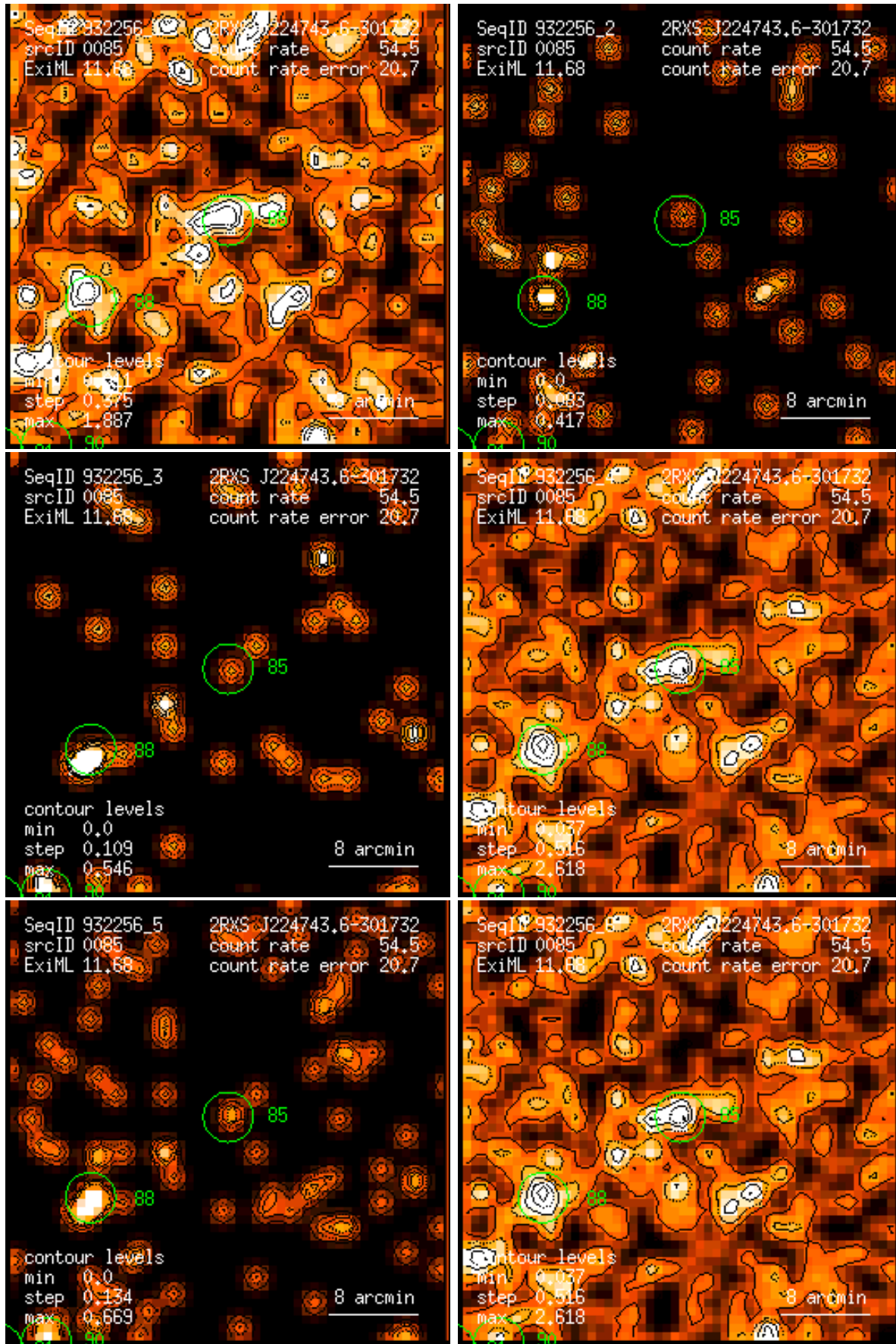
Figure 85: RASS 932256: detection 0085: band rate images, Gaussian filter: (1) PSPC channels 11 – 41, (2) 52 – 90, (3) 91 – 201, (4) 11 – 235, (5) 52 – 201, (6) 11 – 201. Broad band rates in counts/ks. Band rate contour levels in counts/ks/arcmin 2 .
