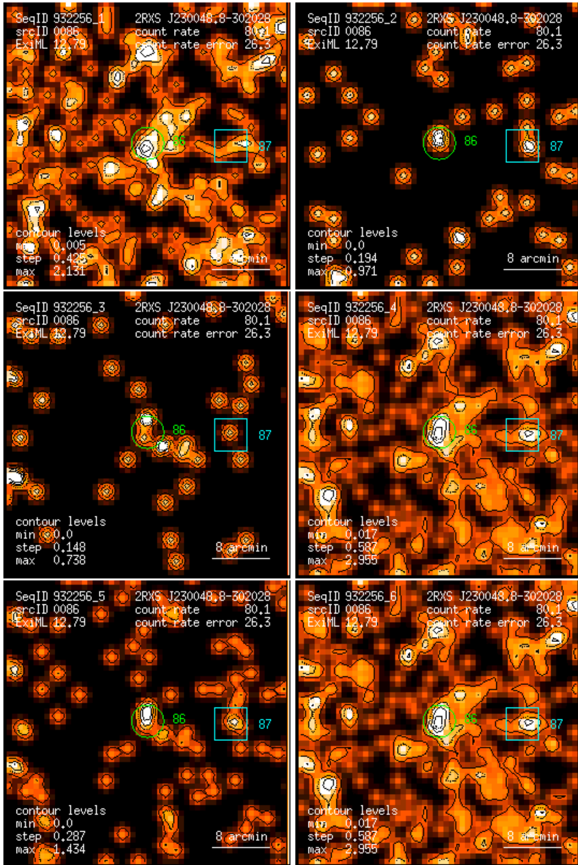
Figure 86: RASS 932256: detection 0086: band rate images, Gaussian filter: (1) PSPC channels 11 – 41, (2) 52 – 90, (3) 91 – 201, (4) 11 – 235, (5) 52 – 201, (6) 11 – 201. Broad band rates in counts/ks. Band rate contour levels in counts/ks/arcmin 2 .
