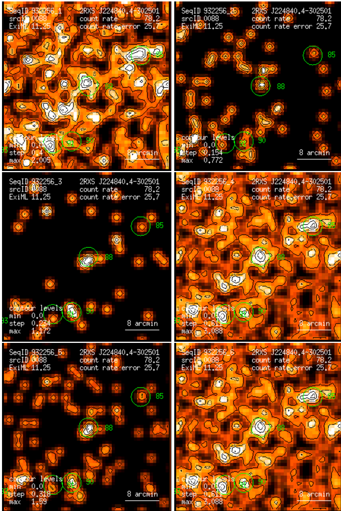
Figure 88: RASS 932256: detection 0088: band rate images, Gaussian filter: (1) PSPC channels 11 – 41, (2) 52 – 90, (3) 91 – 201, (4) 11 – 235, (5) 52 – 201, (6) 11 – 201. Broad band rates in counts/ks. Band rate contour levels in counts/ks/arcmin 2 .
