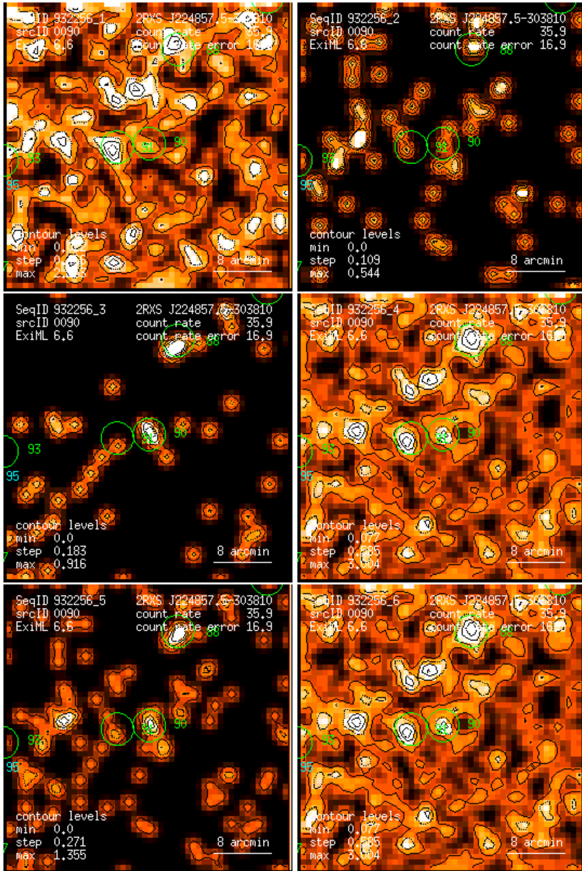
Figure 90: RASS 932256: detection 0090: band rate images, Gaussian filter: (1) PSPC channels 11 – 41, (2) 52 – 90, (3) 91 – 201, (4) 11 – 235, (5) 52 – 201, (6) 11 – 201. Broad band rates in counts/ks. Band rate contour levels in counts/ks/arcmin 2 .
