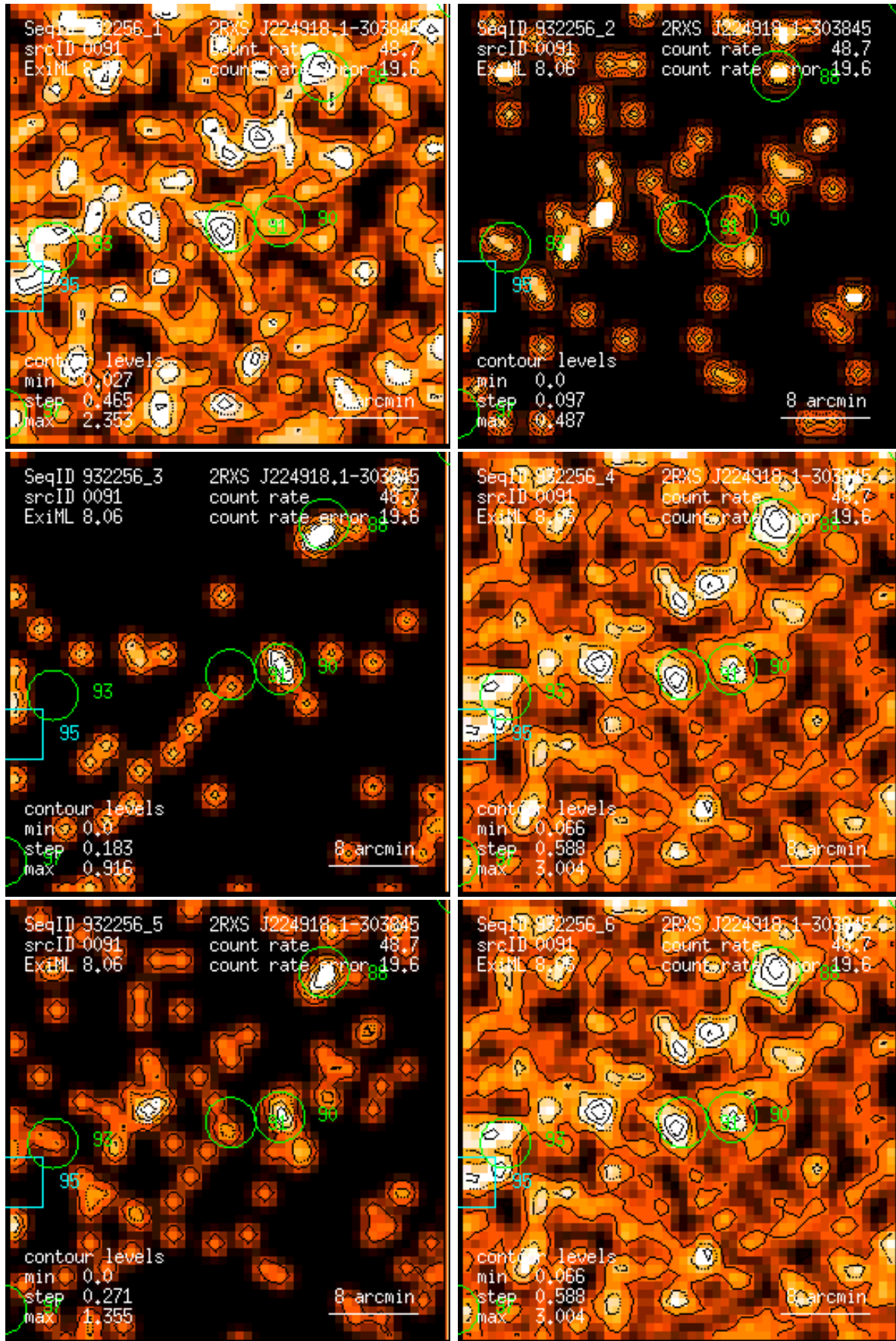
Figure 91: RASS 932256: detection 0091: band rate images, Gaussian filter: (1) PSPC channels 11 – 41, (2) 52 – 90, (3) 91 – 201, (4) 11 – 235, (5) 52 – 201, (6) 11 – 201. Broad band rates in counts/ks. Band rate contour levels in counts/ks/arcmin 2 .
