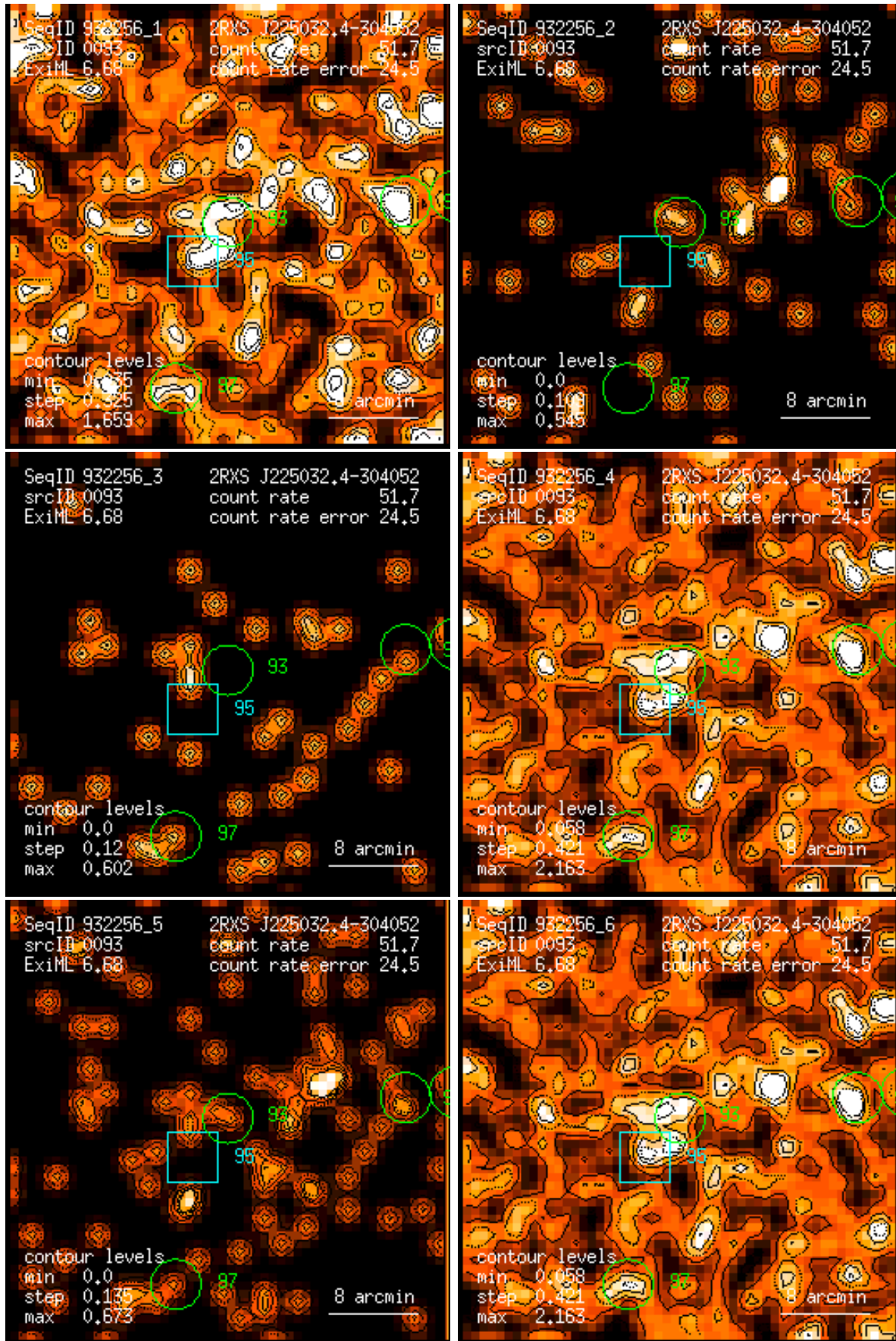
Figure 93: RASS 932256: detection 0093: band rate images, Gaussian filter: (1) PSPC channels 11 – 41, (2) 52 – 90, (3) 91 – 201, (4) 11 – 235, (5) 52 – 201, (6) 11 – 201. Broad band rates in counts/ks. Band rate contour levels in counts/ks/arcmin 2 .
