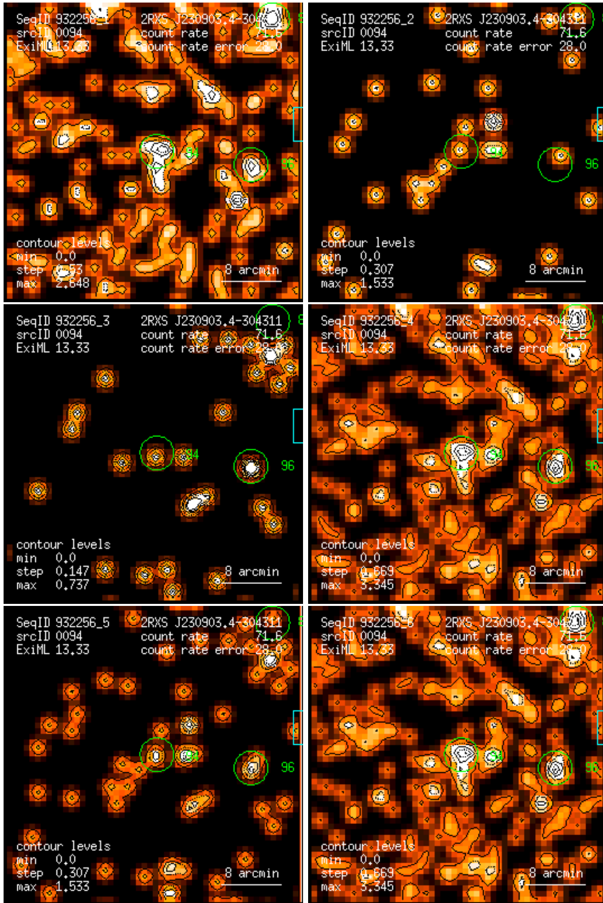
Figure 94: RASS 932256: detection 0094: band rate images, Gaussian filter: (1) PSPC channels 11 – 41, (2) 52 – 90, (3) 91 – 201, (4) 11 – 235, (5) 52 – 201, (6) 11 – 201. Broad band rates in counts/ks. Band rate contour levels in counts/ks/arcmin 2 .
