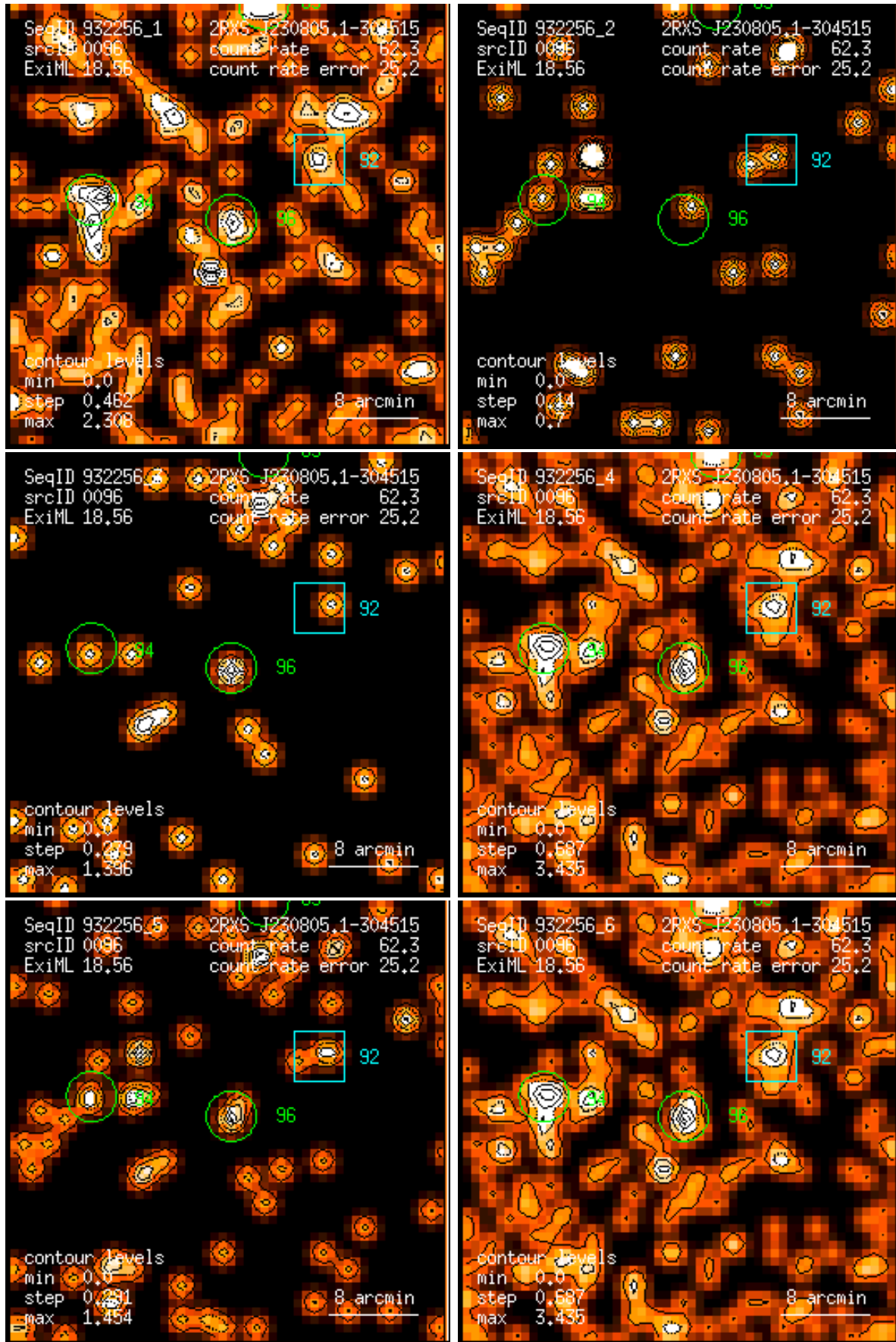
Figure 96: RASS 932256: detection 0096: band rate images, Gaussian filter: (1) PSPC channels 11 – 41, (2) 52 – 90, (3) 91 – 201, (4) 11 – 235, (5) 52 – 201, (6) 11 – 201. Broad band rates in counts/ks. Band rate contour levels in counts/ks/arcmin 2 .
