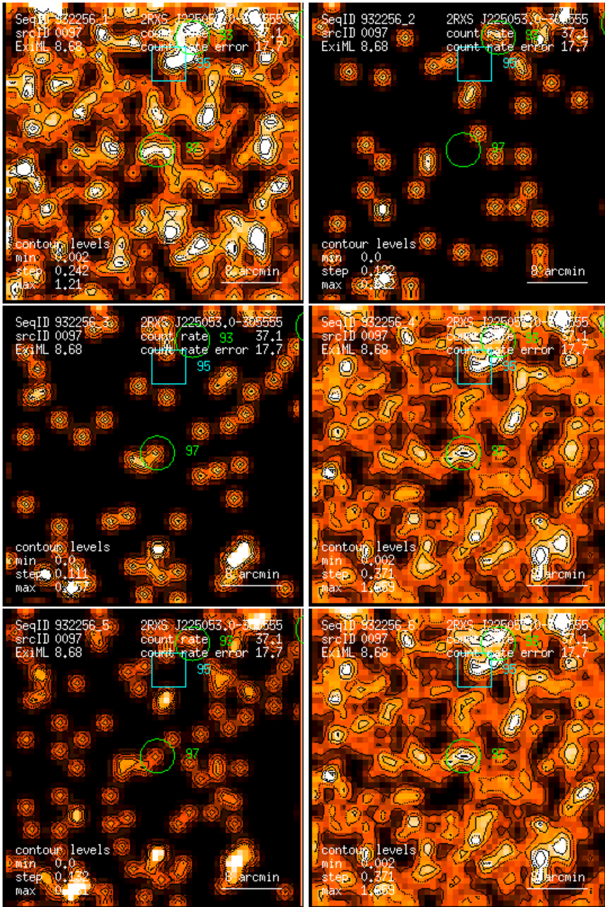
Figure 97: RASS 932256: detection 0097: band rate images, Gaussian filter: (1) PSPC channels 11 – 41, (2) 52 – 90, (3) 91 – 201, (4) 11 – 235, (5) 52 – 201, (6) 11 – 201. Broad band rates in counts/ks. Band rate contour levels in counts/ks/arcmin 2 .
