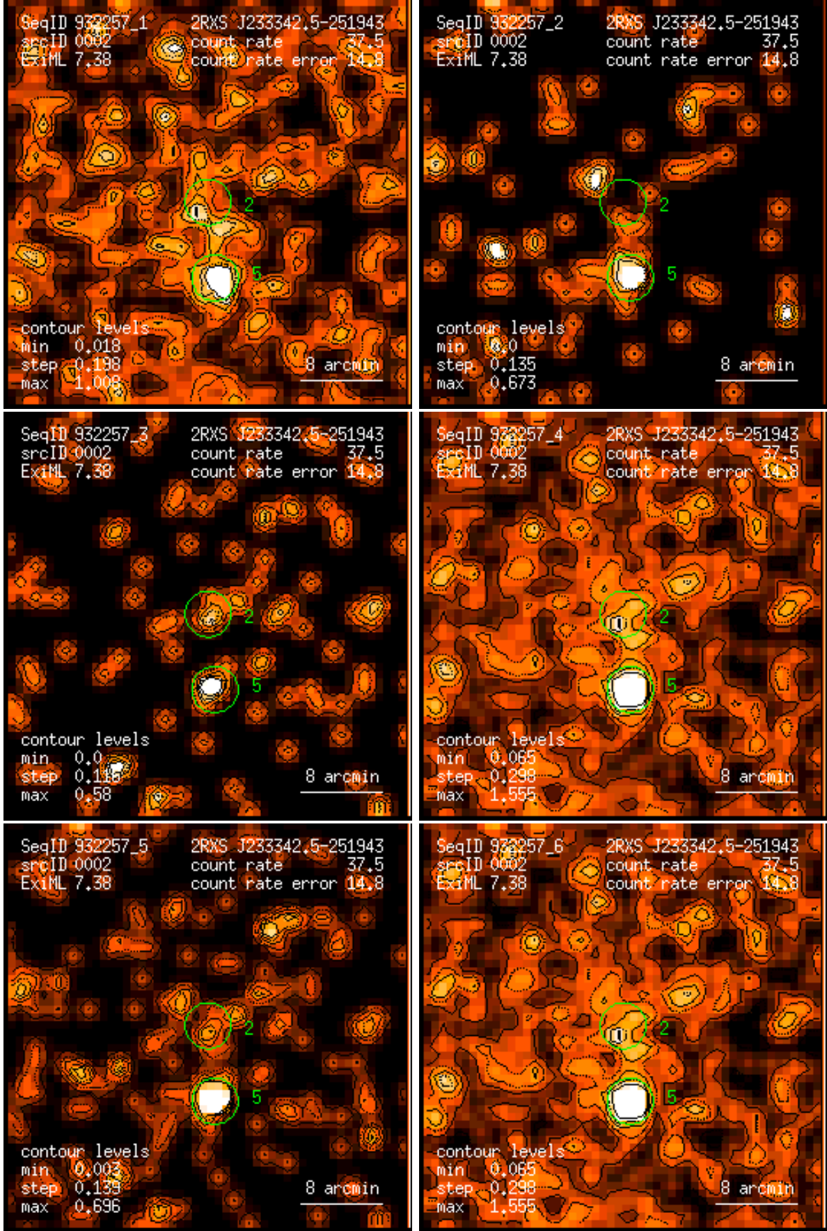
Figure 2: RASS 932257: detection 0002: band rate images, Gaussian filter: (1) PSPC channels 11 – 41, (2) 52 – 90, (3) 91 – 201, (4) 11 – 235, (5) 52 – 201, (6) 11 – 201. Broad band rates in counts/ks. Band rate contour levels in counts/ks/arcmin 2 .
