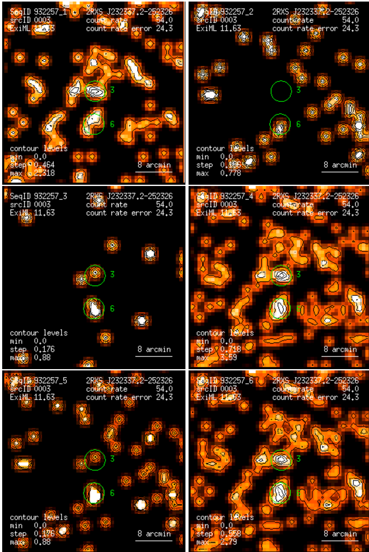
Figure 3: RASS 932257: detection 0003: band rate images, Gaussian filter: (1) PSPC channels 11 – 41, (2) 52 – 90, (3) 91 – 201, (4) 11 – 235, (5) 52 – 201, (6) 11 – 201. Broad band rates in counts/ks. Band rate contour levels in counts/ks/arcmin 2 .
