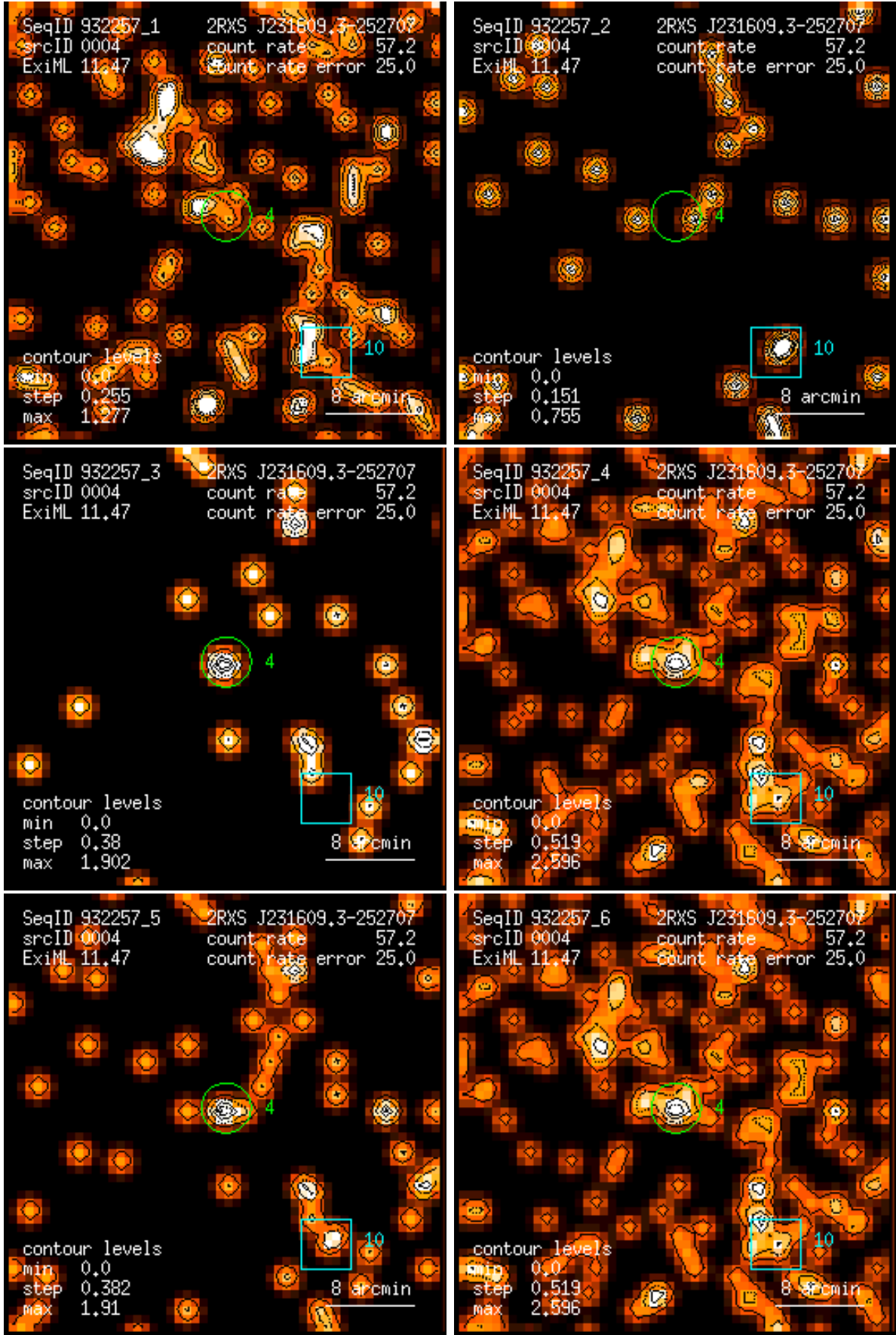
Figure 4: RASS 932257: detection 0004: band rate images, Gaussian filter: (1) PSPC channels 11 – 41, (2) 52 – 90, (3) 91 – 201, (4) 11 – 235, (5) 52 – 201, (6) 11 – 201. Broad band rates in counts/ks. Band rate contour levels in counts/ks/arcmin 2 .
