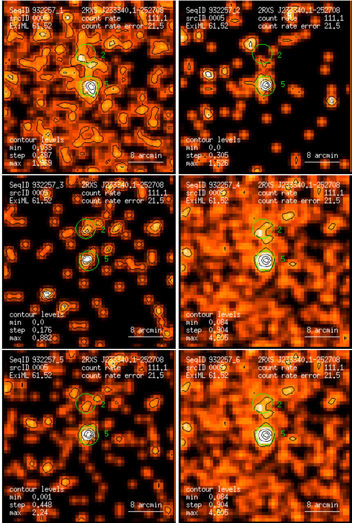
Figure 5: RASS 932257: detection 0005: band rate images, Gaussian filter: (1) PSPC channels 11 – 41, (2) 52 – 90, (3) 91 – 201, (4) 11 – 235, (5) 52 – 201, (6) 11 – 201. Broad band rates in counts/ks. Band rate contour levels in counts/ks/arcmin 2 .
