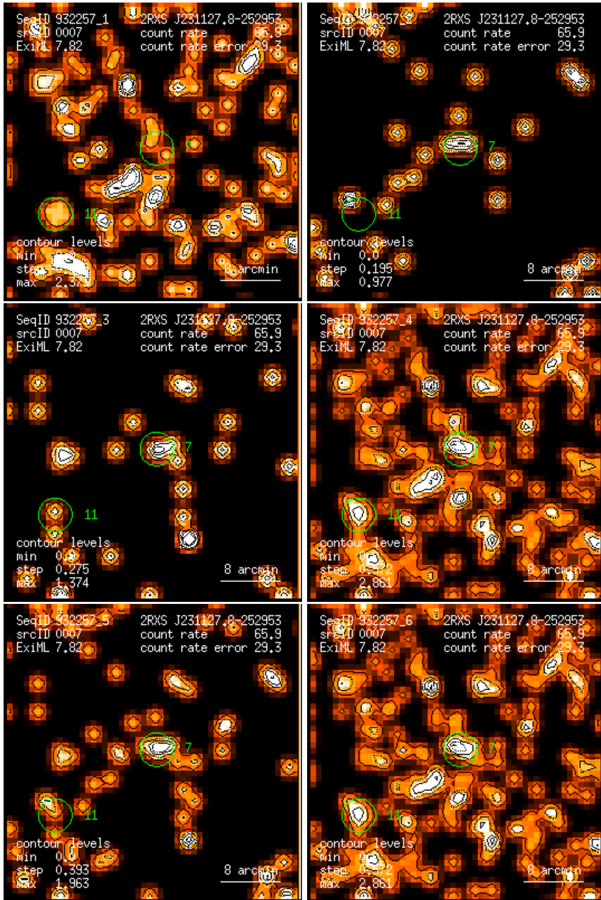
Figure 7: RASS 932257: detection 0007: band rate images, Gaussian filter: (1) PSPC channels 11 – 41, (2) 52 – 90, (3) 91 – 201, (4) 11 – 235, (5) 52 – 201, (6) 11 – 201. Broad band rates in counts/ks. Band rate contour levels in counts/ks/arcmin 2 .
