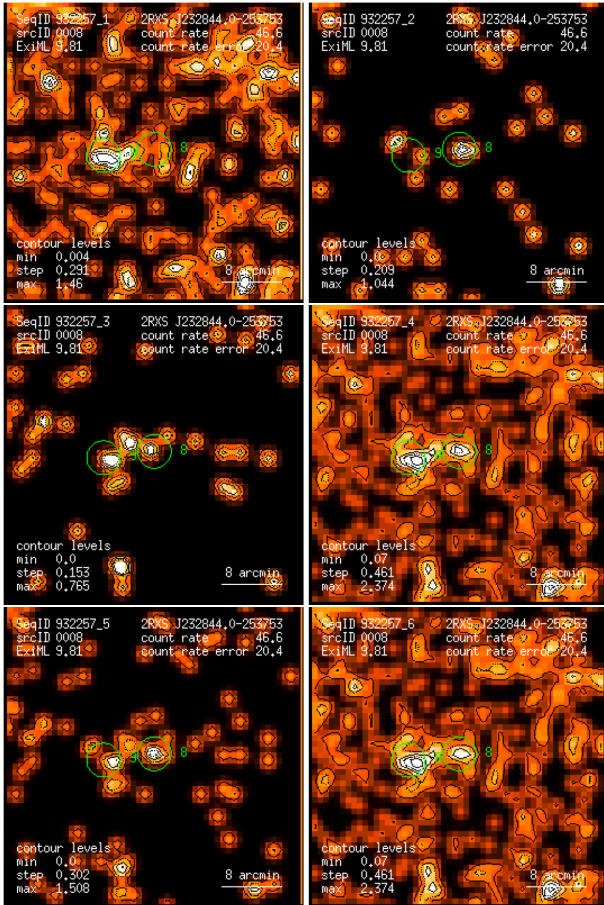
Figure 8: RASS 932257: detection 0008: band rate images, Gaussian filter: (1) PSPC channels 11 – 41, (2) 52 – 90, (3) 91 – 201, (4) 11 – 235, (5) 52 – 201, (6) 11 – 201. Broad band rates in counts/ks. Band rate contour levels in counts/ks/arcmin 2 .
