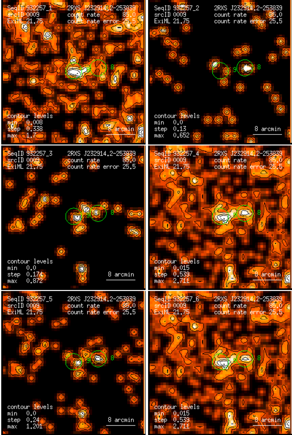
Figure 9: RASS 932257: detection 0009: band rate images, Gaussian filter: (1) PSPC channels 11 – 41, (2) 52 – 90, (3) 91 – 201, (4) 11 – 235, (5) 52 – 201, (6) 11 – 201. Broad band rates in counts/ks. Band rate contour levels in counts/ks/arcmin 2 .
