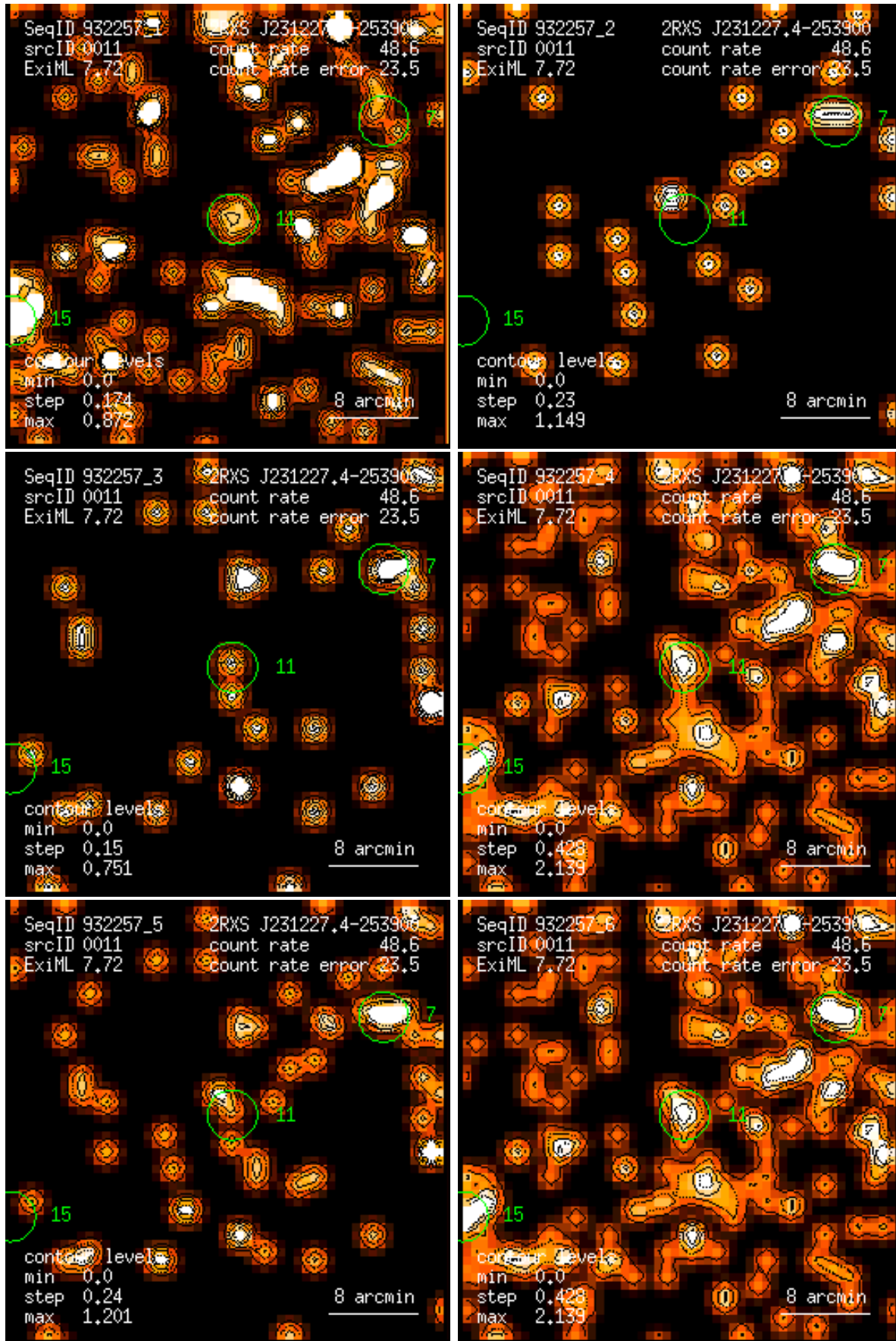
Figure 11: RASS 932257: detection 0011: band rate images, Gaussian filter: (1) PSPC channels 11 – 41, (2) 52 – 90, (3) 91 – 201, (4) 11 – 235, (5) 52 – 201, (6) 11 – 201. Broad band rates in counts/ks. Band rate contour levels in counts/ks/arcmin 2 .
