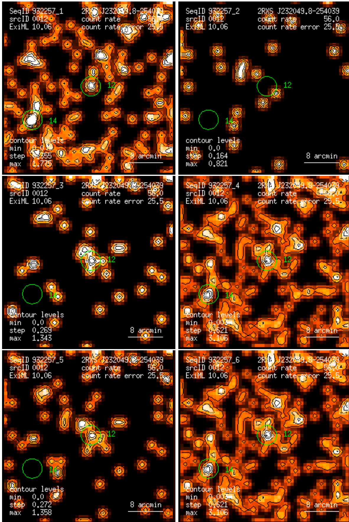
Figure 12: RASS 932257: detection 0012: band rate images, Gaussian filter: (1) PSPC channels 11 – 41, (2) 52 – 90, (3) 91 – 201, (4) 11 – 235, (5) 52 – 201, (6) 11 – 201. Broad band rates in counts/ks. Band rate contour levels in counts/ks/arcmin 2 .
