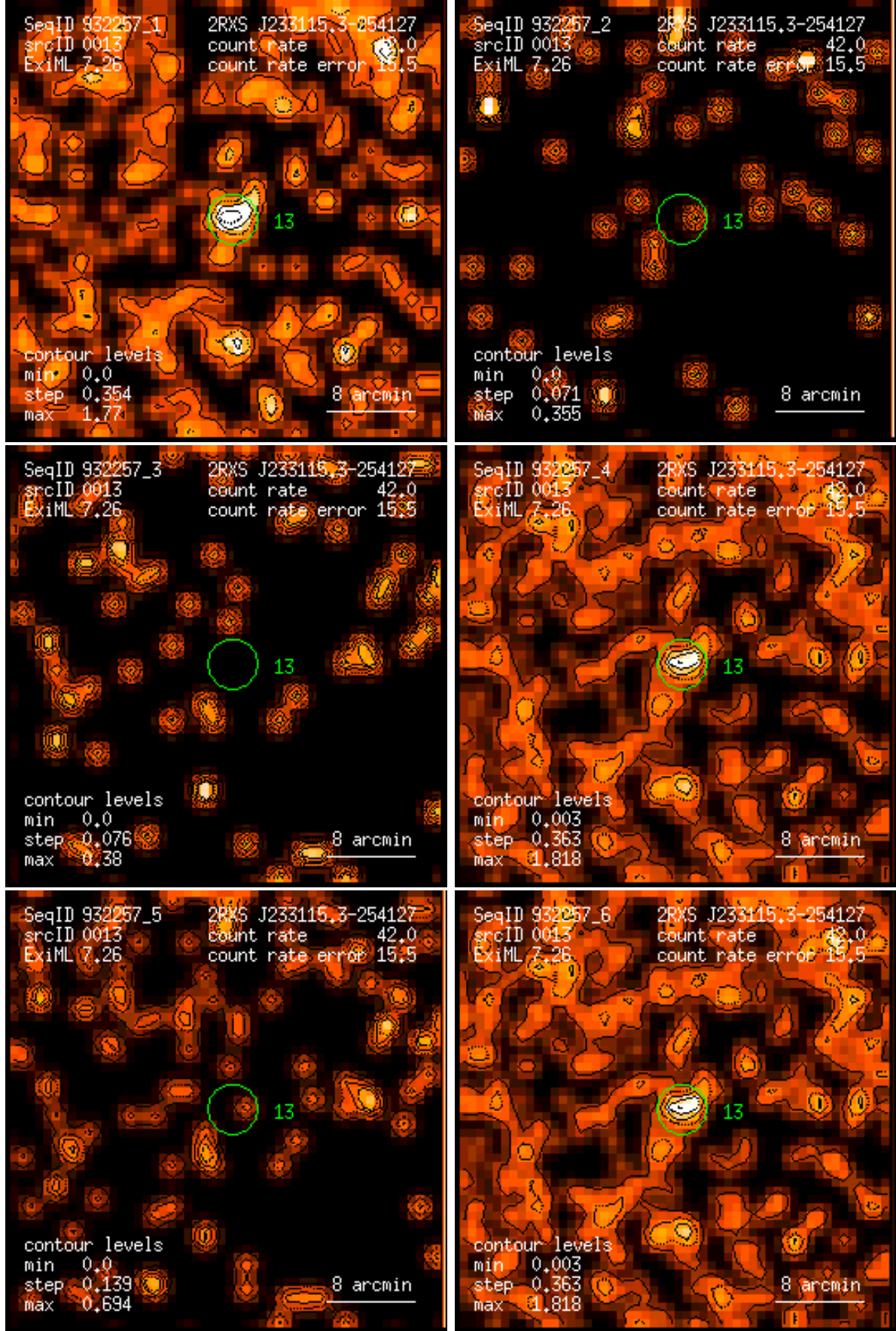
Figure 13: RASS 932257: detection 0013: band rate images, Gaussian filter: (1) PSPC channels 11 – 41, (2) 52 – 90, (3) 91 – 201, (4) 11 – 235, (5) 52 – 201, (6) 11 – 201. Broad band rates in counts/ks. Band rate contour levels in counts/ks/arcmin 2 .
