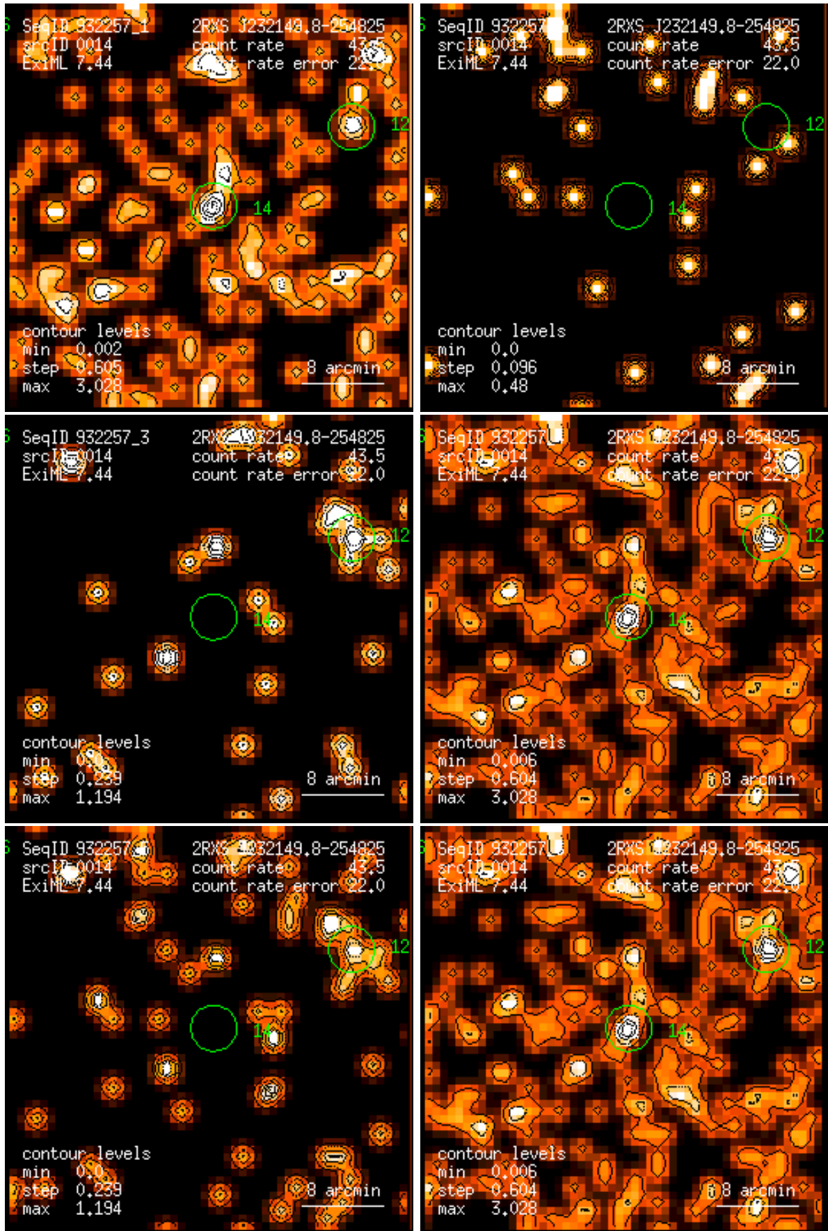
Figure 14: RASS 932257: detection 0014: band rate images, Gaussian filter: (1) PSPC channels 11 – 41, (2) 52 – 90, (3) 91 – 201, (4) 11 – 235, (5) 52 – 201, (6) 11 – 201. Broad band rates in counts/ks. Band rate contour levels in counts/ks/arcmin 2 .
