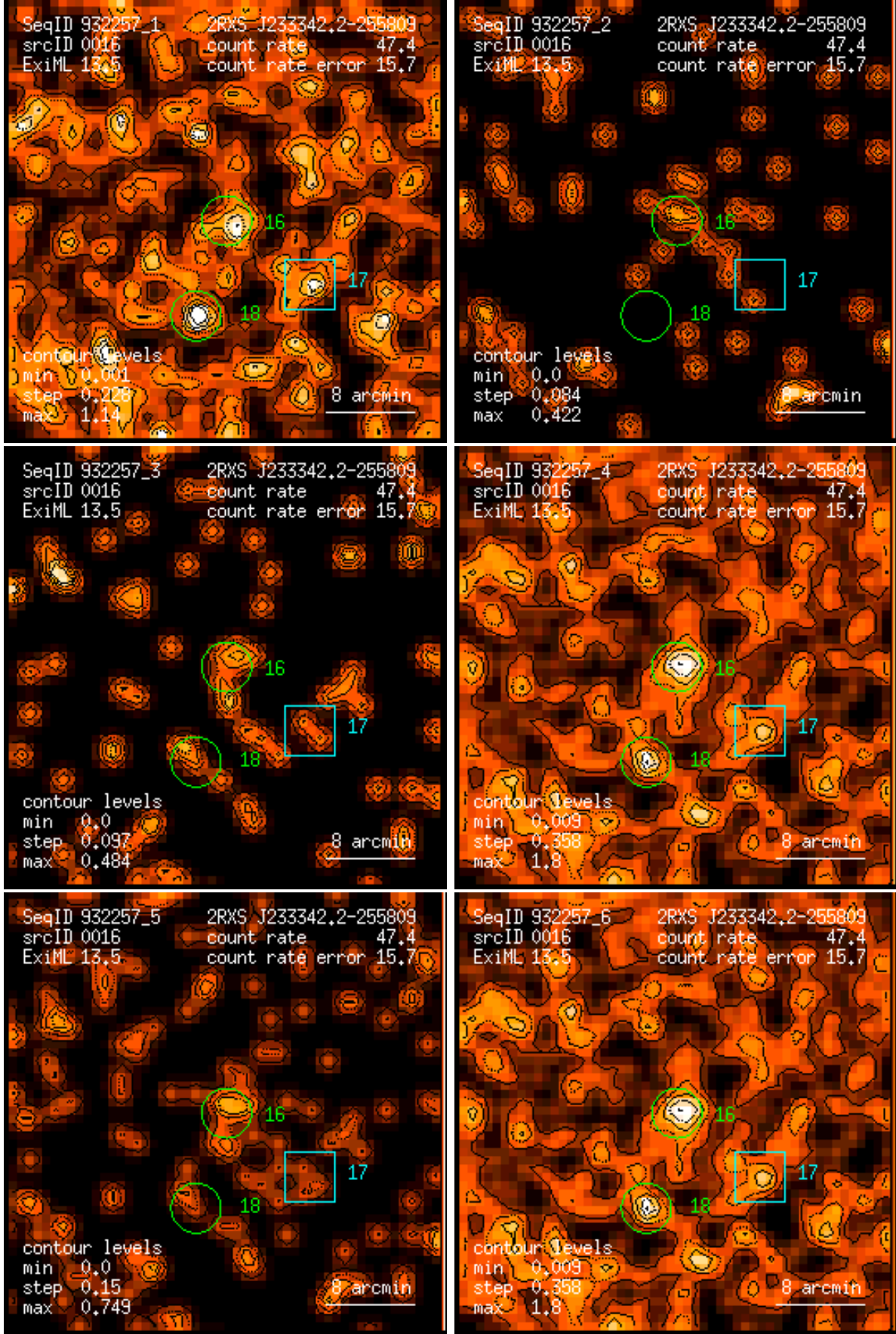
Figure 16: RASS 932257: detection 0016: band rate images, Gaussian filter: (1) PSPC channels 11 – 41, (2) 52 – 90, (3) 91 – 201, (4) 11 – 235, (5) 52 – 201, (6) 11 – 201. Broad band rates in counts/ks. Band rate contour levels in counts/ks/arcmin 2 .
