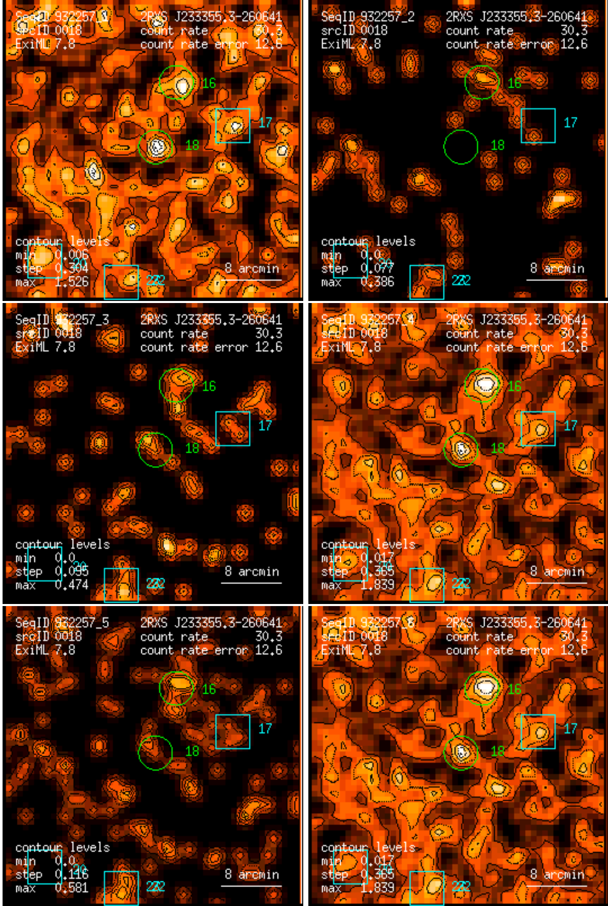
Figure 18: RASS 932257: detection 0018: band rate images, Gaussian filter: (1) PSPC channels 11 – 41, (2) 52 – 90, (3) 91 – 201, (4) 11 – 235, (5) 52 – 201, (6) 11 – 201. Broad band rates in counts/ks. Band rate contour levels in counts/ks/arcmin 2 .
