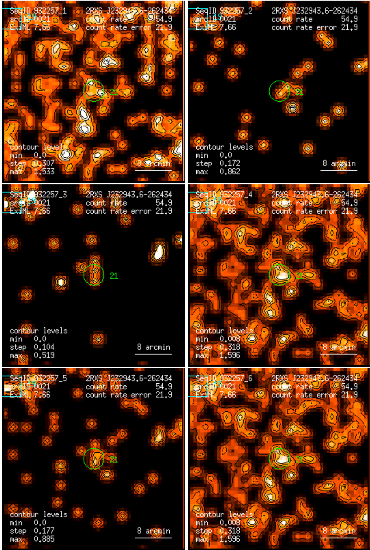
Figure 21: RASS 932257: detection 0021: band rate images, Gaussian filter: (1) PSPC channels 11 – 41, (2) 52 – 90, (3) 91 – 201, (4) 11 – 235, (5) 52 – 201, (6) 11 – 201. Broad band rates in counts/ks. Band rate contour levels in counts/ks/arcmin 2 .
