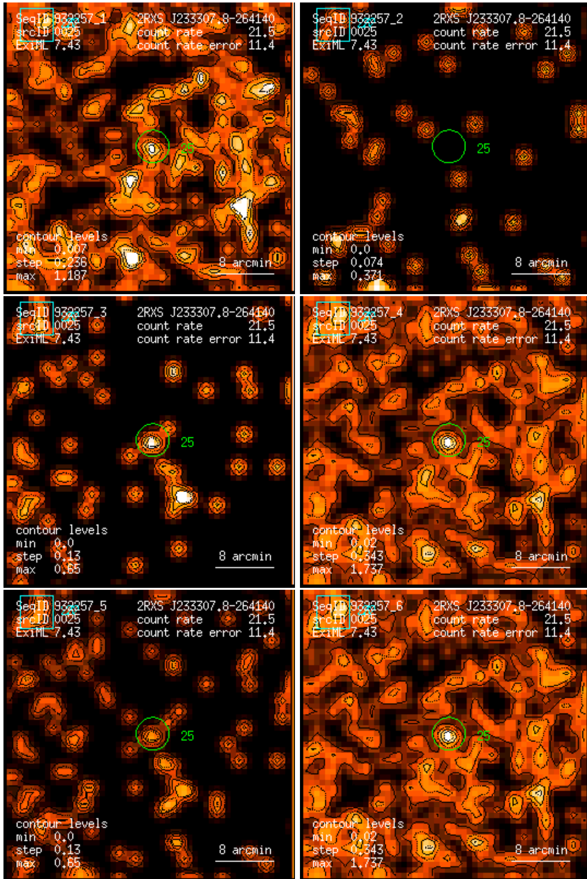
Figure 25: RASS 932257: detection 0025: band rate images, Gaussian filter: (1) PSPC channels 11 – 41, (2) 52 – 90, (3) 91 – 201, (4) 11 – 235, (5) 52 – 201, (6) 11 – 201. Broad band rates in counts/ks. Band rate contour levels in counts/ks/arcmin 2 .
