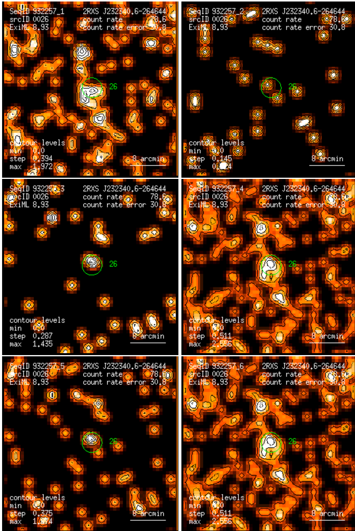
Figure 26: RASS 932257: detection 0026: band rate images, Gaussian filter: (1) PSPC channels 11 – 41, (2) 52 – 90, (3) 91 – 201, (4) 11 – 235, (5) 52 – 201, (6) 11 – 201. Broad band rates in counts/ks. Band rate contour levels in counts/ks/arcmin 2 .
