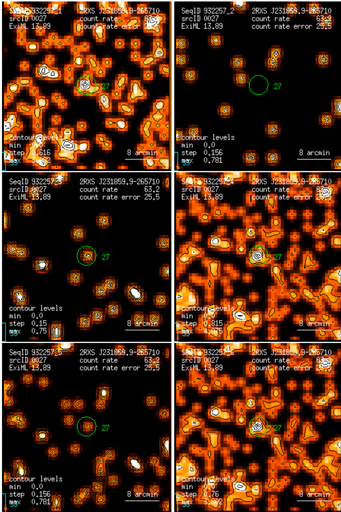
Figure 27: RASS 932257: detection 0027: band rate images, Gaussian filter: (1) PSPC channels 11 – 41, (2) 52 – 90, (3) 91 – 201, (4) 11 – 235, (5) 52 – 201, (6) 11 – 201. Broad band rates in counts/ks. Band rate contour levels in counts/ks/arcmin 2 .
