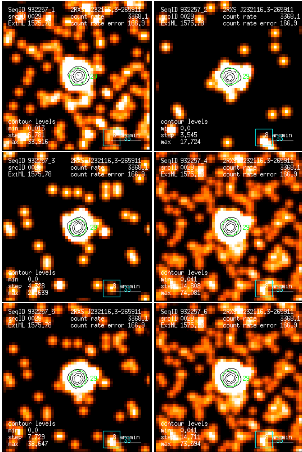
Figure 29: RASS 932257: detection 0029: band rate images, Gaussian filter: (1) PSPC channels 11 – 41, (2) 52 – 90, (3) 91 – 201, (4) 11 – 235, (5) 52 – 201, (6) 11 – 201. Broad band rates in counts/ks. Band rate contour levels in counts/ks/arcmin 2 .
