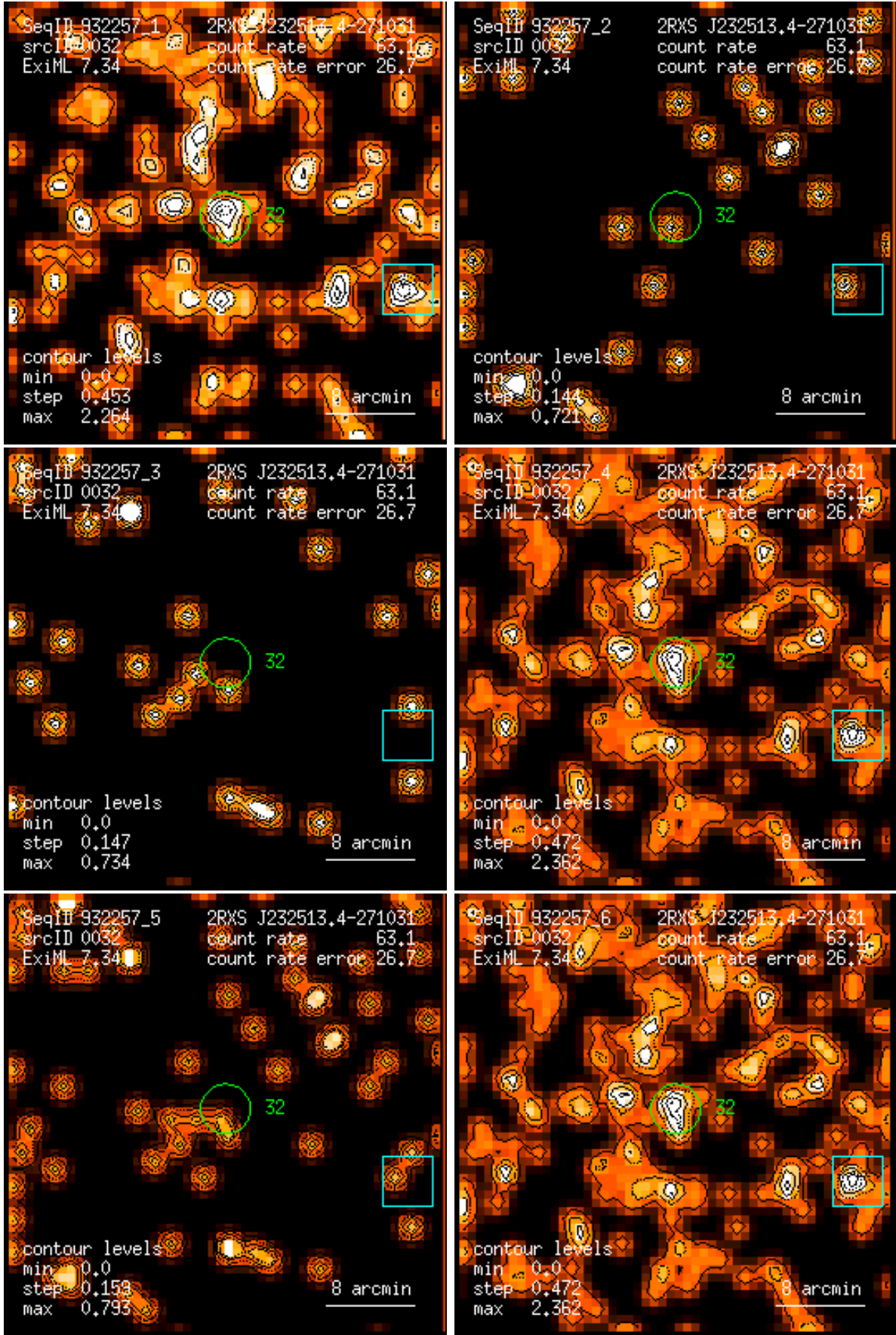
Figure 32: RASS 932257: detection 0032: band rate images, Gaussian filter: (1) PSPC channels 11 – 41, (2) 52 – 90, (3) 91 – 201, (4) 11 – 235, (5) 52 – 201, (6) 11 – 201. Broad band rates in counts/ks. Band rate contour levels in counts/ks/arcmin 2 .
